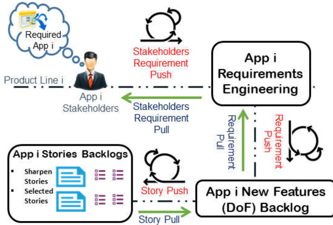
Figure 5 Problem space of Application Engineering in AgiFPL
