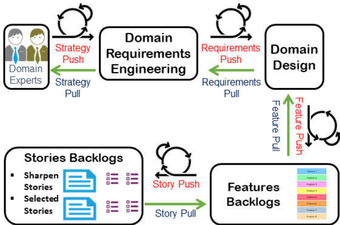
Figure 4 Problem space of Domain Engineering in AgiFPL
