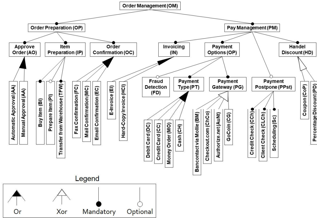
Figure 3 Correspondent Feature Model
