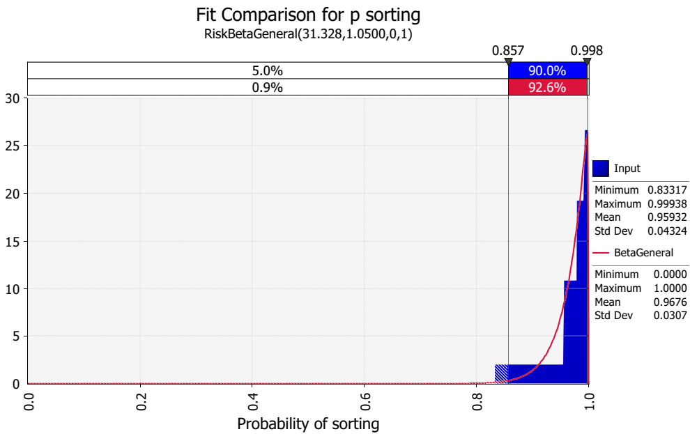
Figure 4: Fitted distribution for sorting ( p_{\text{sorting}} ) as the proportion of infested fruit (both scenarios)
