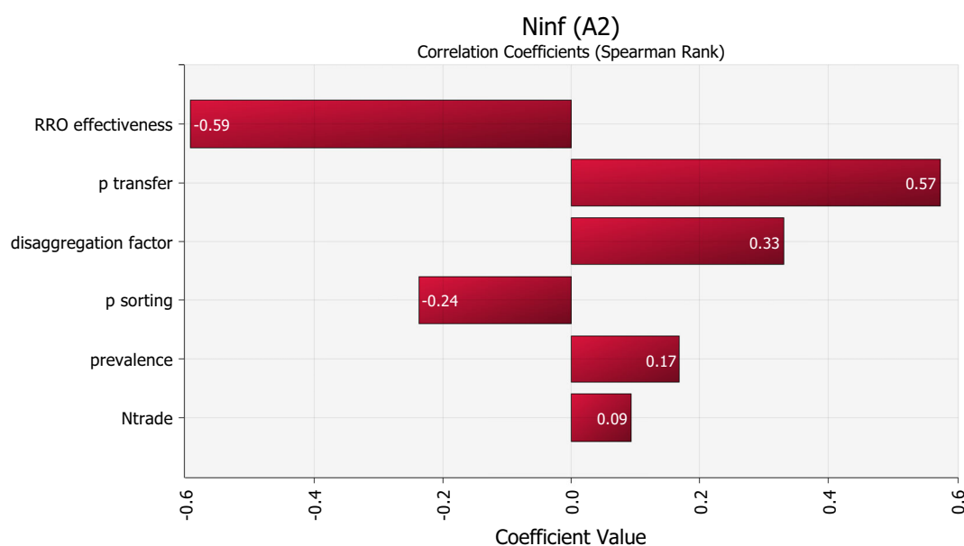
Figure 11: Correlation between the output variable ( N_{inf} ) of the parameters of the entry pathway model for scenario A2 (additional RROs). RRO effectiveness and p_{sorting} have negative correlation coefficients, as they are inserted in the model as (1 - \text{RRO effectiveness}) and (1 - p_{sorting}) .
