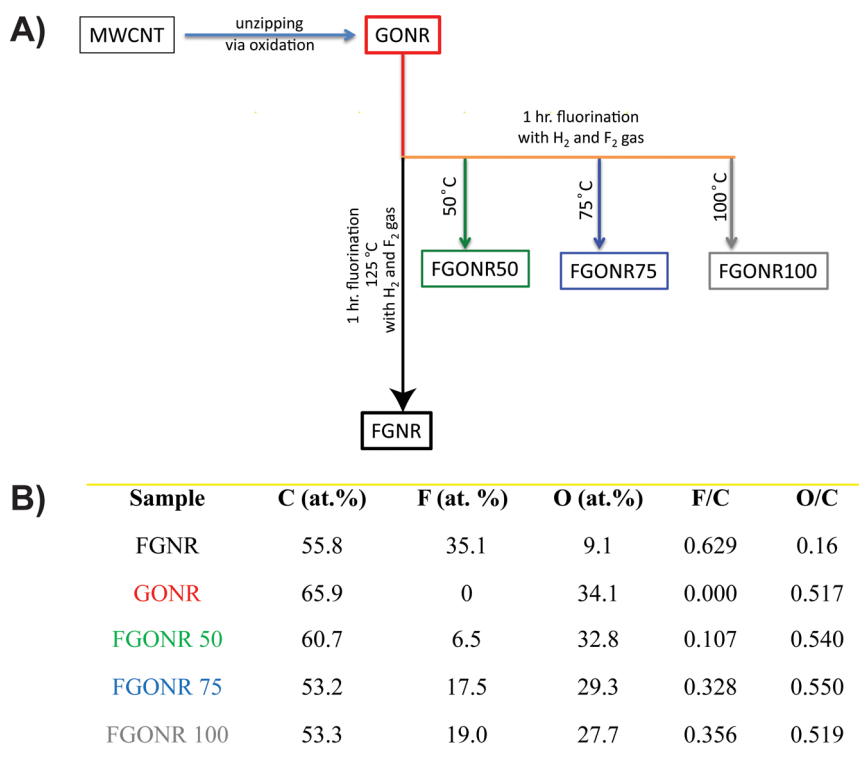
Figure 1. Synthesis of fluorinated graphene oxide nanoribbons (FGONRs) and their XPS elemental analysis. (A) Graphical representation of the synthesis mechanism. (B) Elemental analysis of GONR, FGNR, and FGONRs 50, 75, and 100.
