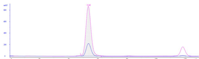
Figure S3. Size exclusion chromatography of VT750-rhDNase (a) and VT750-PEG30-rhDNase (b) using HiLoad Superdex 200 pg column. Labelled proteins were eluted with 150 mM NaCl and 1 mM CaCl 2 at 1 mL/min. Elution was monitored by measuring the absorbance at 280 nm (blue) and 700 nm (magenta). The retention times are 80.0 ml for VT750-rhDNase, 53.6 ml for VT750-PEG30-rhDNase, and around 118 ml for the unreacted dye (VT750).
