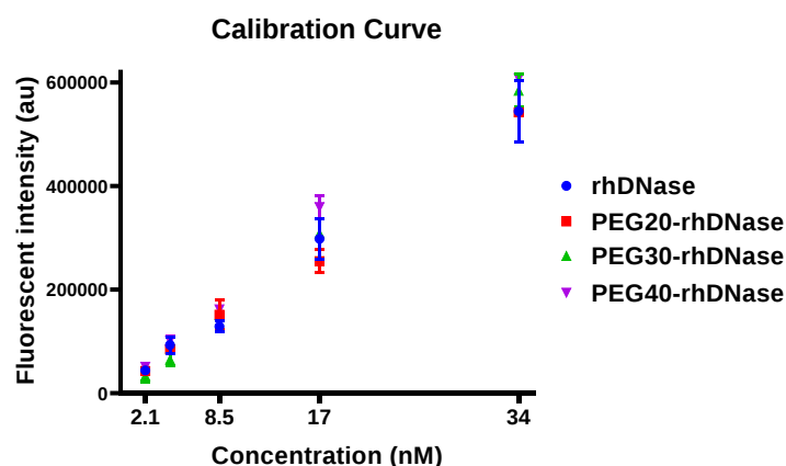
Figure S2. Calibration curves of rhodamine labelled rhDNase and PEGylated rhDNase in 1 mM \text{CaCl}_2 150 mM NaCl buffer. Fluorescence was measured in dark 96 well plate at wavelength 555/580 nm for excitation and emission.
