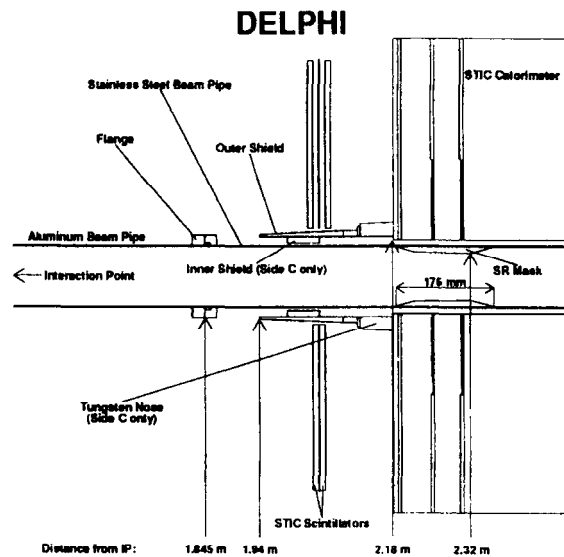
Fig. 3. Layout of the STIC region.
