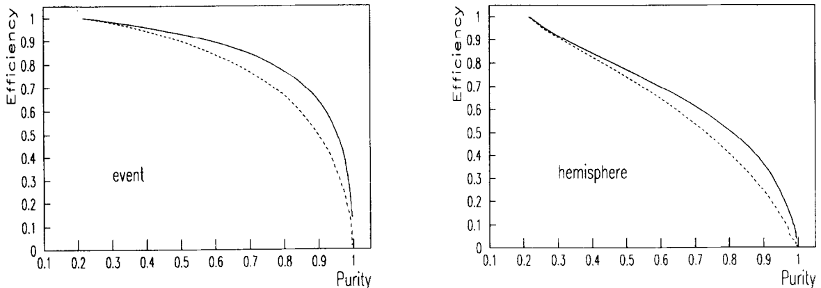
Fig. 15. b-tagging efficiencies as a function of the purity of the tagged sample for different values of the cut on the event probability (left) and on the hemisphere probability (right) for the 3-coordinates VD providing Rz information (full line) and the 2-coordinates VD that provided only R\phi information (dashed line).
