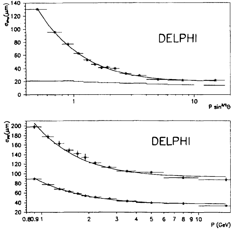
Fig. 13. Upper: Mean track extrapolation uncertainty in R\phi measured as a function of p \sin^{3/2} \theta ( p in GeV/c). The values are determined by subtracting quadratically the vertex position uncertainty, shown by the bottom curve, from the measured impact parameter uncertainty. The full line depicts (65/p \sin^{3/2} \theta \oplus 20) \mu\text{m} . Lower: Mean track extrapolation uncertainty in the Rz plane, measured similarly as a function of the particle momentum. The two curves correspond to tracks with 80^\circ < \theta < 90^\circ (bottom) and 45^\circ < \theta < 55^\circ (top). The full lines depict (71/p \oplus 39) \mu\text{m} and (151/p \oplus 96) \mu\text{m} respectively.
