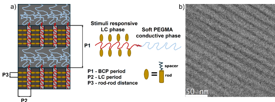
Figure 4. Hierarchical morphology of LC-containing BCPs and BCPs. (a) Scheme depicting the proposed structure, where LCs anchor homogeneously with respect to the BCP intermaterial dividing surface, resulting in the perpendicular orientation of the smectic layer. (b) TEM micrograph depicting the lam-in-LAM microstructure of S1_Salt/DC with LC layer spacing P2 of 3 nm.
