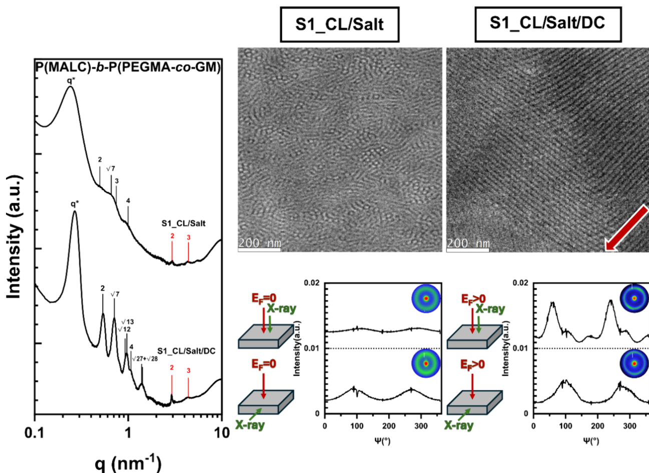
Figure 3. SAXS and TEM data of crosslinked S1 doped with salt in the various casting set-ups. Left: 1D scattering profiles integrated from I_0 \parallel E_F measurement. Top right: TEM micrographs of corresponding microstructures. Bottom right: I(\Psi) profiles with 2D inserts from I_0 \parallel E_F and I_0 \perp E_F acquisitions. The red arrow indicates the direction of the E_F .
