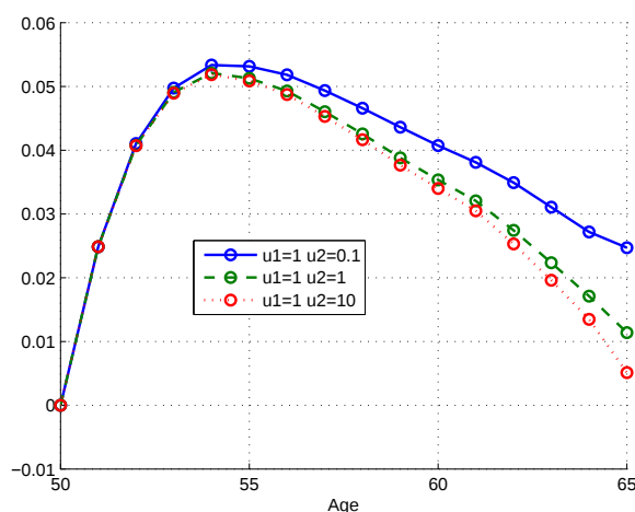
Figure 6.7.2: -UL_t (% of the fund).
