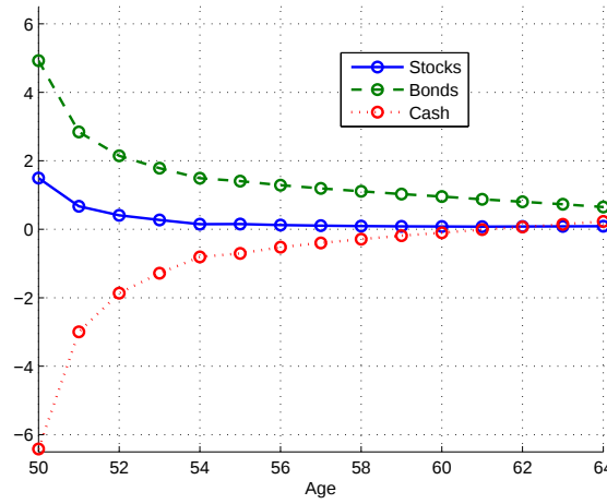
Figure 6.7.3: Asset mix for u_1 = 1 and u_2 = 10 .
