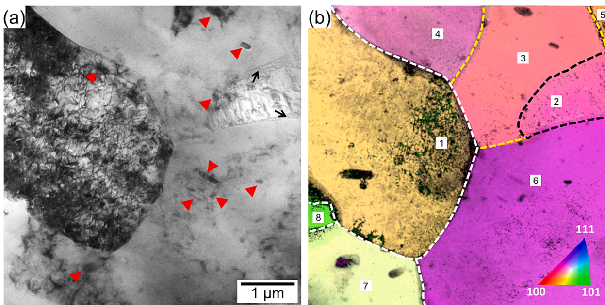
Fig. 2. Structure of Al-0.5Mg 2 Si alloy in the as-FSP state: (a) BF-TEM image, (b) IPF map of the same location overlaid with cross-correlation index and reliability. HAGBs, LAGBs, and SGBs are indicated by white, yellow, and black lines, respectively. Black arrows point to dislocation walls and red triangular markers point to precipitates. (For interpretation of the references to colour in this figure legend, the reader is referred to the web version of this article.)
