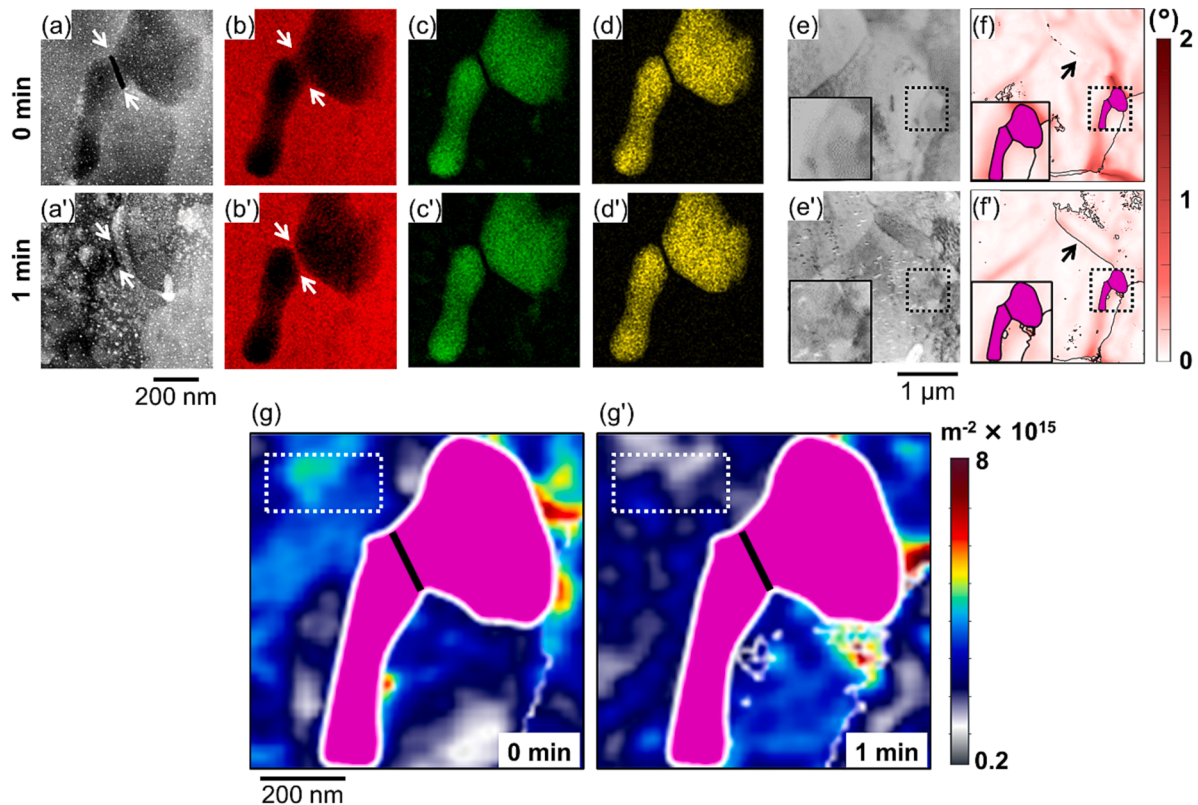
Fig. 7. Analysis of the healing process in Al-0.5Mg 2 Si alloy based on in situ TEM heating in combination with STEM-EDX ((a)-(d)) and ACOM-TEM ((e)-(g)) in the initial or pre-healed state: (a) HAADF-STEM image with arrows pointing to the crack, (b) Al-map, (c) Mg-map, (d) Si-map, (e) BF-STEM with dotted-rectangle showing the exact location of acquisition of the STEM-EDX maps in (a)-(d), in-set shows magnified view of the area within the rectangle, (f) KAM map from the same region seen in (e) and overlaid with Mg 2 Si particle (pink) traced as analyzed using STEM-EDX, in-set shows magnified view of area within the dotted-rectangle, and the location of crack (black segment), and (g) magnified GND map from the dotted-rectangle (in (e)-(f)) with Mg 2 Si particle (pink) and the location of crack (black segment). (a')-(g') are the respective images after 1 min of healing heat treatment at 350 °C. Scale bar for (a)-(a') to (d)-(d') is shown below (a'), for (e)-(e') and (f)-(f') is shown below (e') and for (g)-(g') is shown below (g). The dotted-box in (g)-(g') indicates the region where the local GND is computed. (For interpretation of the references to colour in this figure legend, the reader is referred to the web version of this article.)
