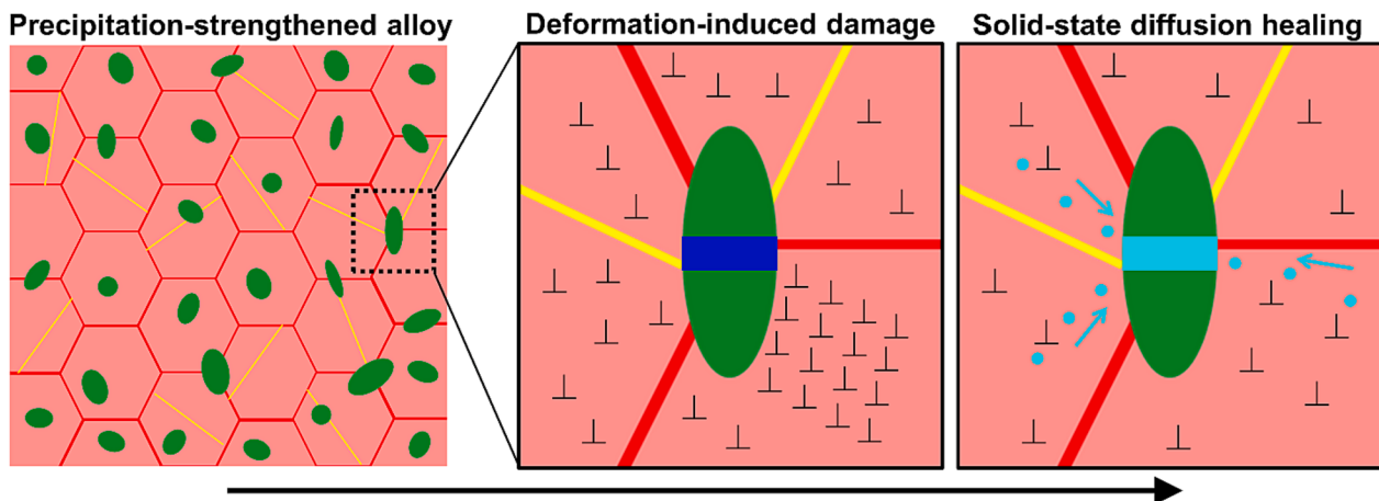
Fig. 1. Principle of the precipitation, damage, and healing mechanism in the PDR alloy which are followed sequentially with reference to the evolution of defects. GBs are in red, SGBs are in yellow and dislocations are schematized inside the matrix (light red). The matrix in the as-prepared state (after FSP) contains precipitates (in green) which lead to precipitation strengthening. Localized damage is introduced by externally applied mechanical load and indicated by a crack (in blue) inside a precipitate. Thermally activated solid-state diffusion healing is schematized by the transfer of fast-diffusing atoms (in aqua) present in the matrix towards the crack leading to its healing and the healed segment is shown in aqua. (For interpretation of the references to colour in this figure legend, the reader is referred to the web version of this article.)
