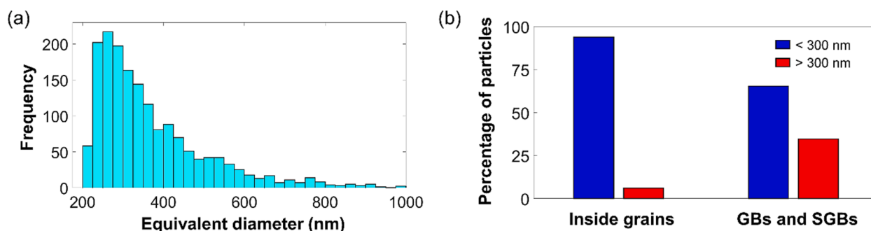
Fig. 4. (a) Particle size distribution of \text{Mg}_2\text{Si} precipitates analyzed from STEM-EDX mapping, (b) localization of the precipitates inside the matrix (inside grain or at GBs or SGBs) categorized into fine (<300 nm) and coarse (>300 nm), analyzed using ACOM-TEM and STEM-EDX mappings.
