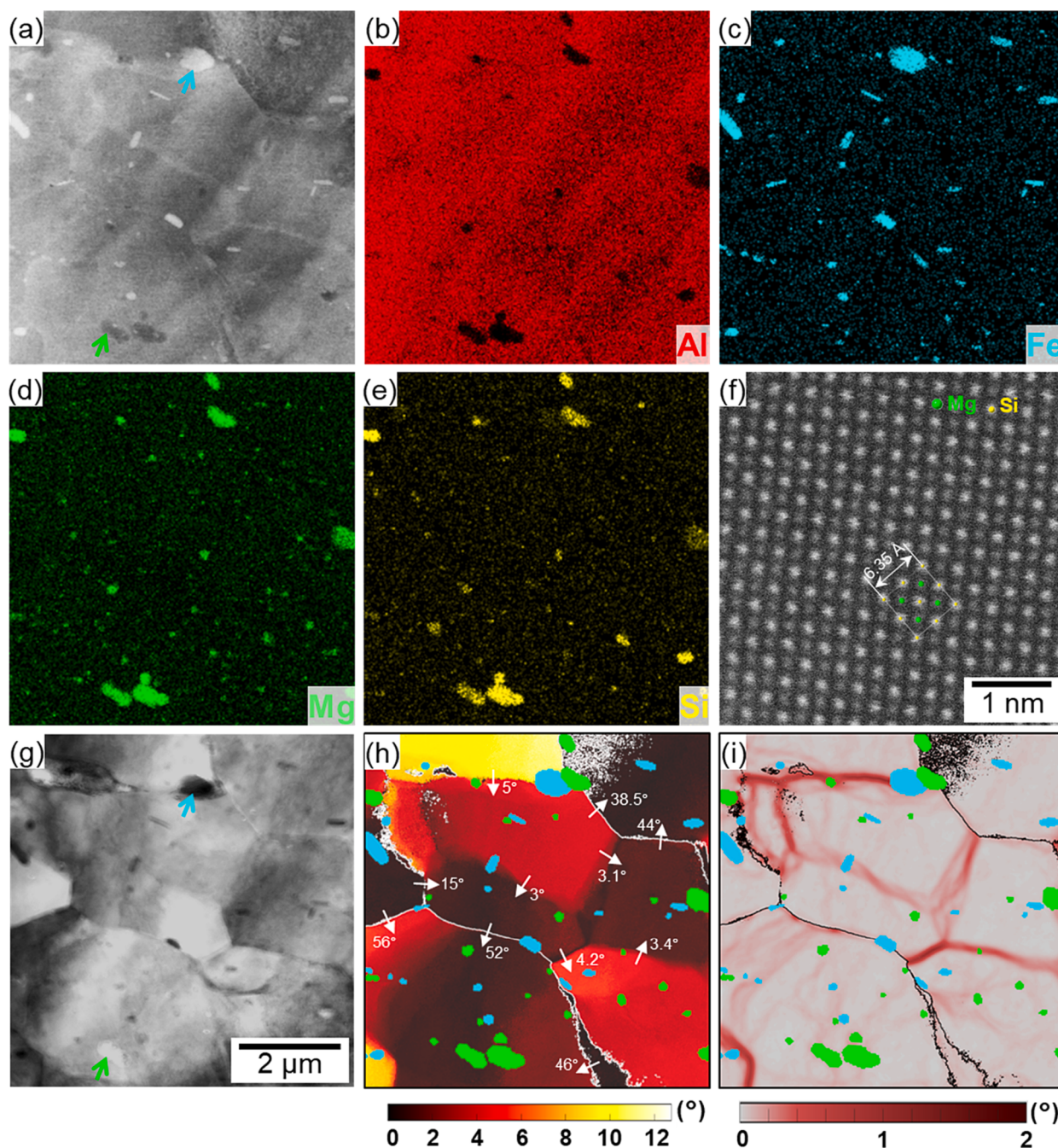
Fig. 3. Analysis of the precipitation behavior based on STEM-EDX and ACOM-TEM: (a) HAADF-STEM image with arrows showing Fe-rich intermetallic (blue) and Mg- and Si-rich particles (green), (b)-(e) elemental maps, (f) HRSTEM image of a \text{Mg}_2\text{Si} precipitate, (g) BF-STEM image with arrows showing Fe-rich intermetallic (blue) and Mg- and Si-rich particles (green) also observable in (a), (h) mis2mean map with GBs (white) with white arrows indicating misorientations at GBs and SGBs, and (i) KAM map with GBs (black) overlaid with Fe-rich (blue) and Mg-rich particles (green). The scale bar for (a)-(e) and (g)-(i) is provided in (g). (For interpretation of the references to colour in this figure legend, the reader is referred to the web version of this article.)
