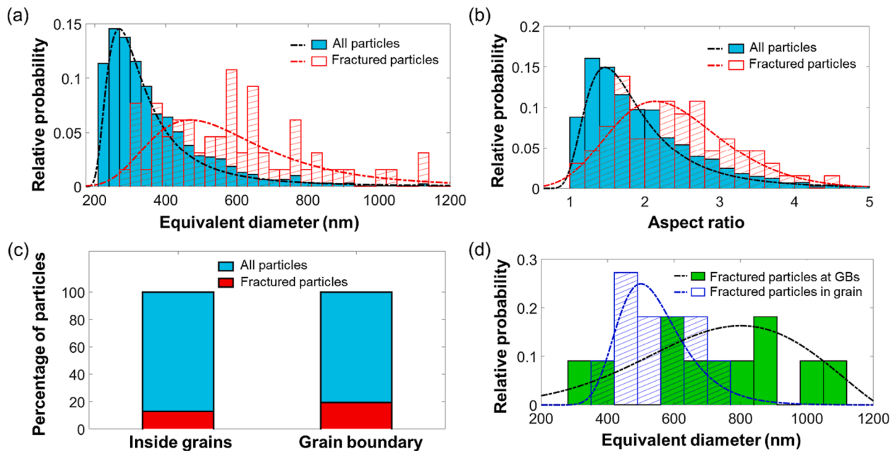
Fig. 6. Statistical analysis of the damaged particles obtained from STEM-EDX and ACOM-TEM analysis: (a) particle size distribution and (b) aspect ratio of damaged particles and all particles fitted with generalized extreme value distribution, (c) distribution of particles in grain and at GBs (HAGBs and LAGBs), and (d) size distribution of particles inside grain and at GBs (HAGBs and LAGBs) fitted with generalized extreme value distribution.
