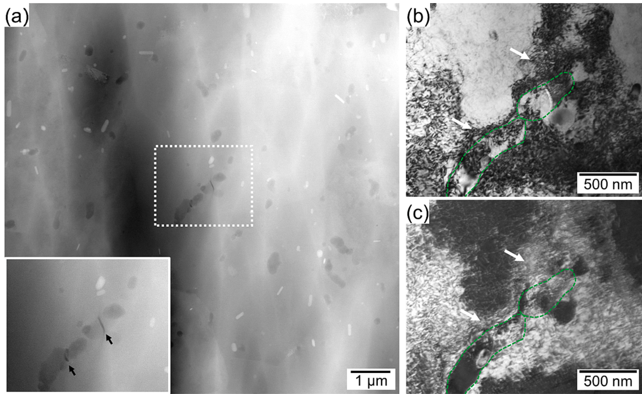
Fig. 5. (a) HAADF-STEM image showing damage indicated by arrows within dotted-box, magnified view shown in the in-set, (b) BF-TEM, and (c) DF-TEM images of cracked \text{Mg}_2\text{Si} particles seen in the box in (a), where green dotted-lines indicate particle-matrix interfaces and white arrows indicate dislocations. (For interpretation of the references to colour in this figure legend, the reader is referred to the web version of this article.)
