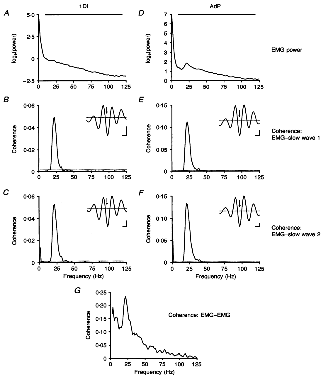
Figure 5. Spectral measures calculated from EMG recordings
