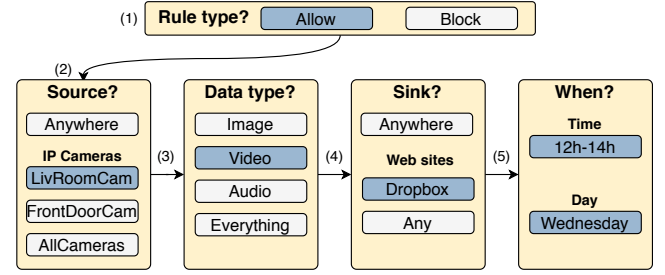
Figure 2. Schematic representation of the UI workflow to specify a privacy rule using dataflow model.
