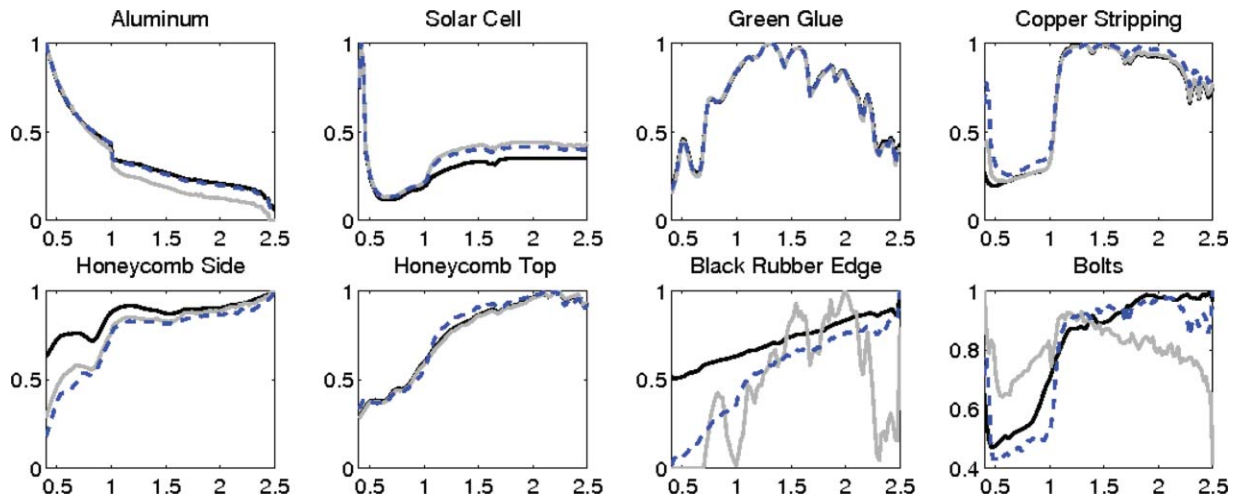
Fig. 15 End-members for the Hubble satellite data with noise and blur. NMU with \ell_2 (gray solid) and NMU with \ell_1 (dashed) versus eight true end-members (black solid).
