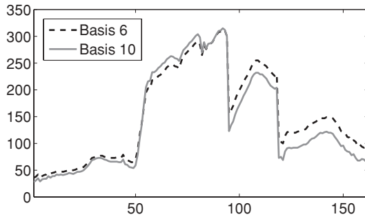
Fig. 9 Spectral signatures of grass: weighted average of the spectral signatures of the pixels present in basis elements 6 and 10 of the \ell_1 -norm solution.
