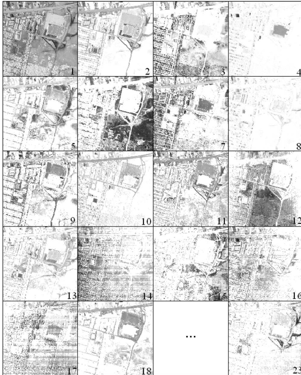
Fig. 5 Basis elements (columns of matrix U ) for the Urban dataset extracted with \ell_2 -NMU. Dark tones indicate a strong presence of a pixel in a cluster (0 is white, 1 black), and numbers indicate the position of the factor in the NMU decomposition.
