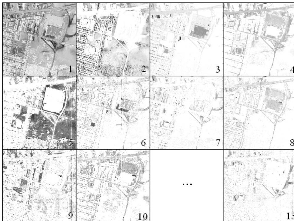
Fig. 10 Basis elements of \ell_2 -NMU for the Urban dataset using only nine bands (bands 1, 20, 40, . . . , 160).
