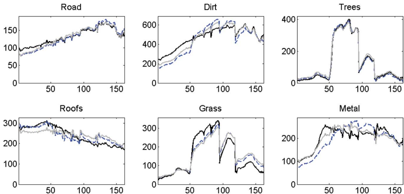
Fig. 8 End-member extraction for the Urban dataset: \ell_2 -NMU (gray solid) and \ell_1 -NMU (dashed) versus six end members from the image using N-FINDR5, 33 plus manual adjustment (dark solid) from Ref. 25. The x-axis gives the wavelength bands while y-axis gives the reflectance values (intensities of reflected light).
