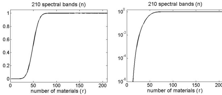
Fig. 1 Probability for at least one column of V' to have one zero element, while another column has a zero at the same position for n = 210 , assuming that (i) V is randomly generated and (ii) V' contains n zeros which are randomly distributed with uniform distribution (with at least one zero by column).
