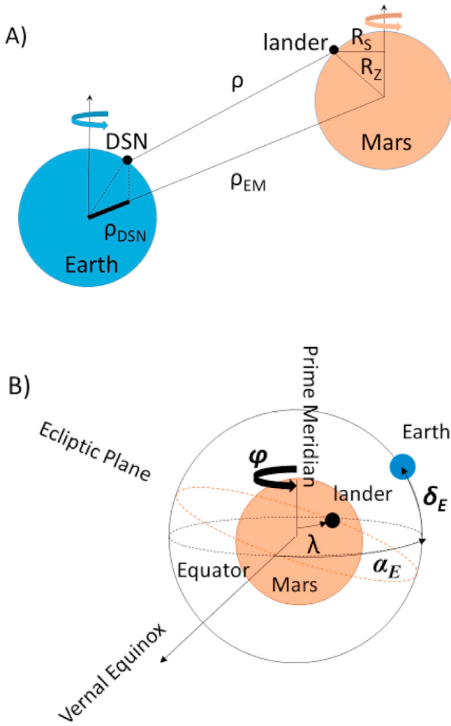
Fig. 1. Geometry for computation of the Doppler shift of a landed asset on Mars.
