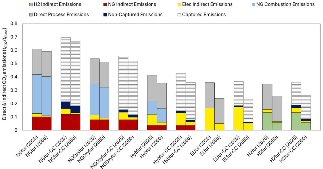
Fig. 3. CO 2 emissions breakdown per tonne of glass across all configurations for 2025 and 2050 scenarios, including direct, indirect and process-related emissions. For CCS-based configurations, captured CO 2 emissions are shown with hatched bars to illustrate the total CO 2 generated and the portion effectively captured.
