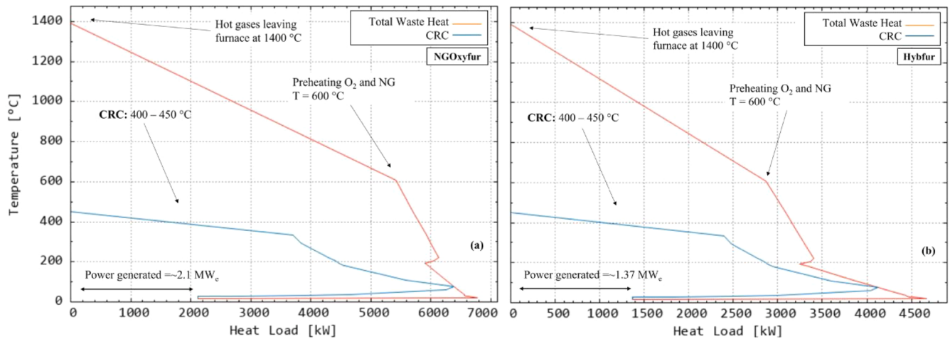
Fig. 5. Integrated composite curves of (a) NGOxyfur configuration and (b) Hybfur configuration, highlighting the power generation potential using a CRC system.
