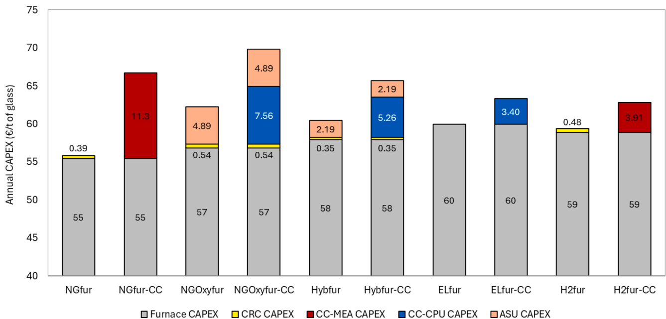
Fig. 8. Breakdown of the annualised CAPEX of all the studied configurations (€/t glass ). Note: The y-axis of the graph starts from 40 €/t glass to highlight the relative incremental burners and additional units' costs.
