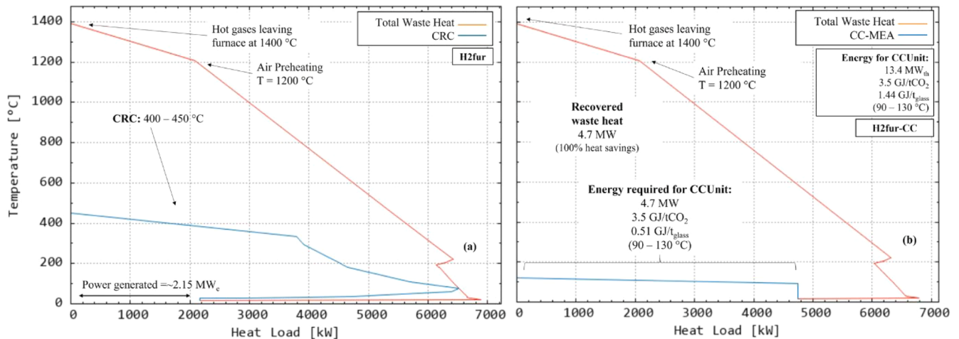
Fig. 6. Integrated composite curves of (a) H2fur configuration recovering waste heat via CRC system and (b) H2fur-CC configuration recovering waste heat for CC-MEA unit.
