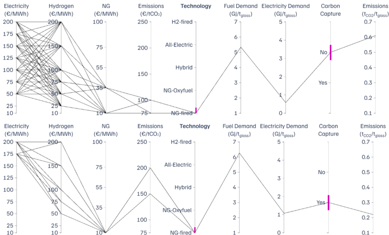
Fig. 11. Parallel coordinates plot depicting the solution space of the NGfur configuration (top) and the NGfur-CC configuration (bottom) as a function of the commodities and CO 2 emissions prices.
