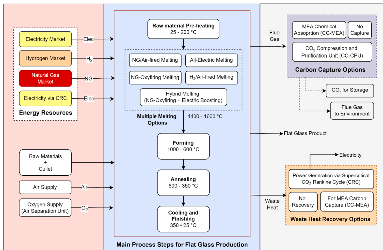
Fig. 2. Superstructure of flat glass production incorporating a comprehensive set of options of energy resources, melting processes, carbon capture units and waste heat recovery methods.
