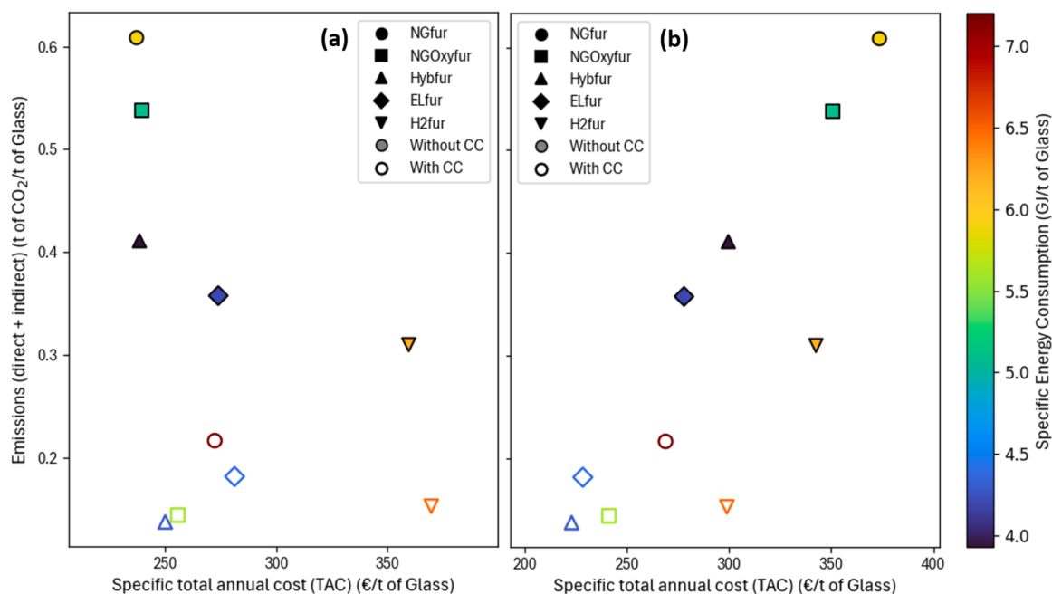
Fig. 10. Pareto plots relating the TAC, CO 2 emissions and specific energy consumption of all the studied configurations for (a) 2025 (left) and (b) 2050 (right) scenarios.
