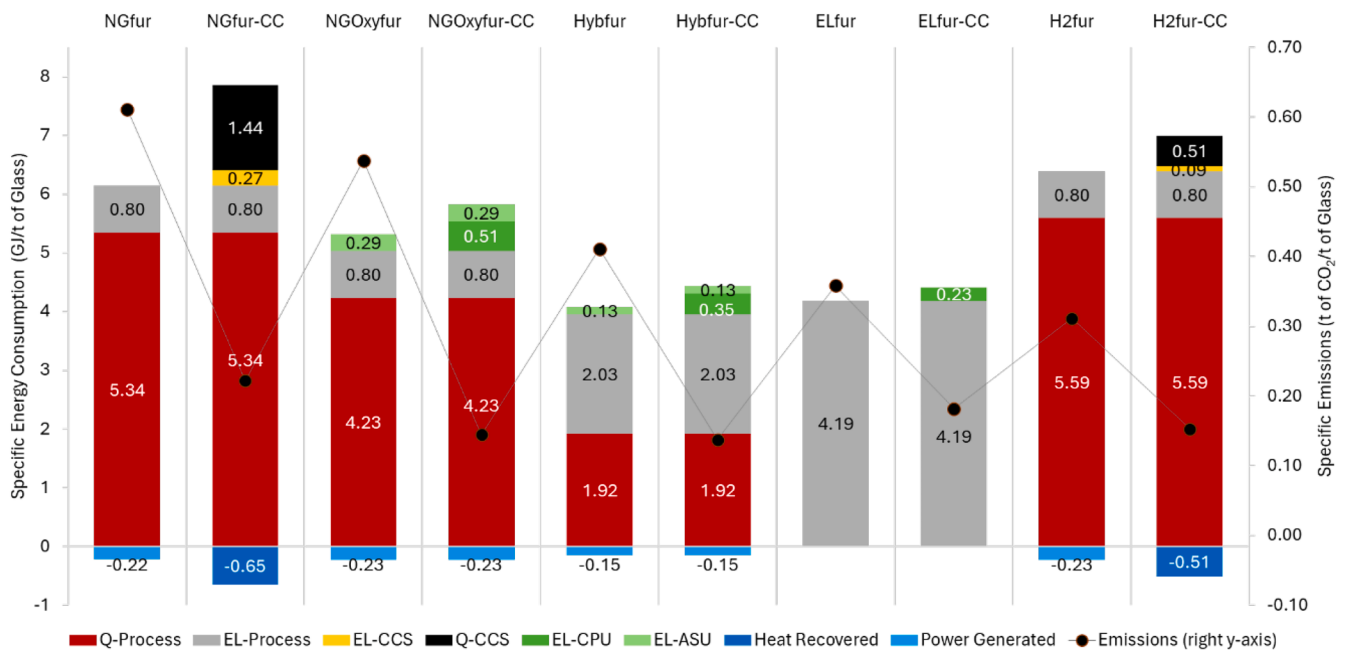
Fig. 7. Energy consumption breakdown (left axis) and total CO 2 emissions (right axis) for all the studied configurations. Q-process and EL-process: heating demand and electricity consumption of the glass process; Q-CCS and EL-CCS: heating demand and electricity consumption of the CC-MEA unit; EL-CPU and EL-ASU: electricity consumption of the CC-CPU and the ASU of the oxy-combustion process; Heat and power recovered: avoided heating and electricity import via waste heat recovery.
