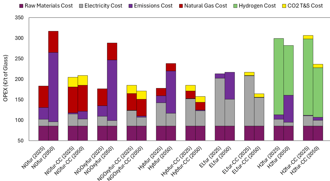
Fig. 9. Breakdown of operational expenses (OPEX) for the studied configurations using commodity prices for 2025 and 2050. Note: The lower bound of y-axis starts at 50 €/t to account for the constant cost of raw materials and to better emphasise the relative contribution of energy commodities.
