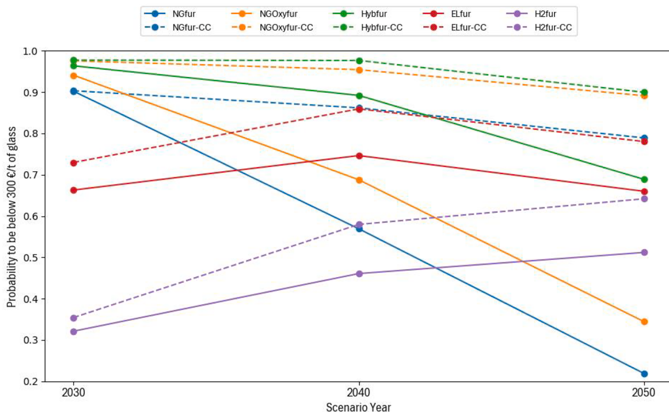
Fig. 17. Probability of each configuration achieving a TAC of 300 €/t glass or lower for each target year.
