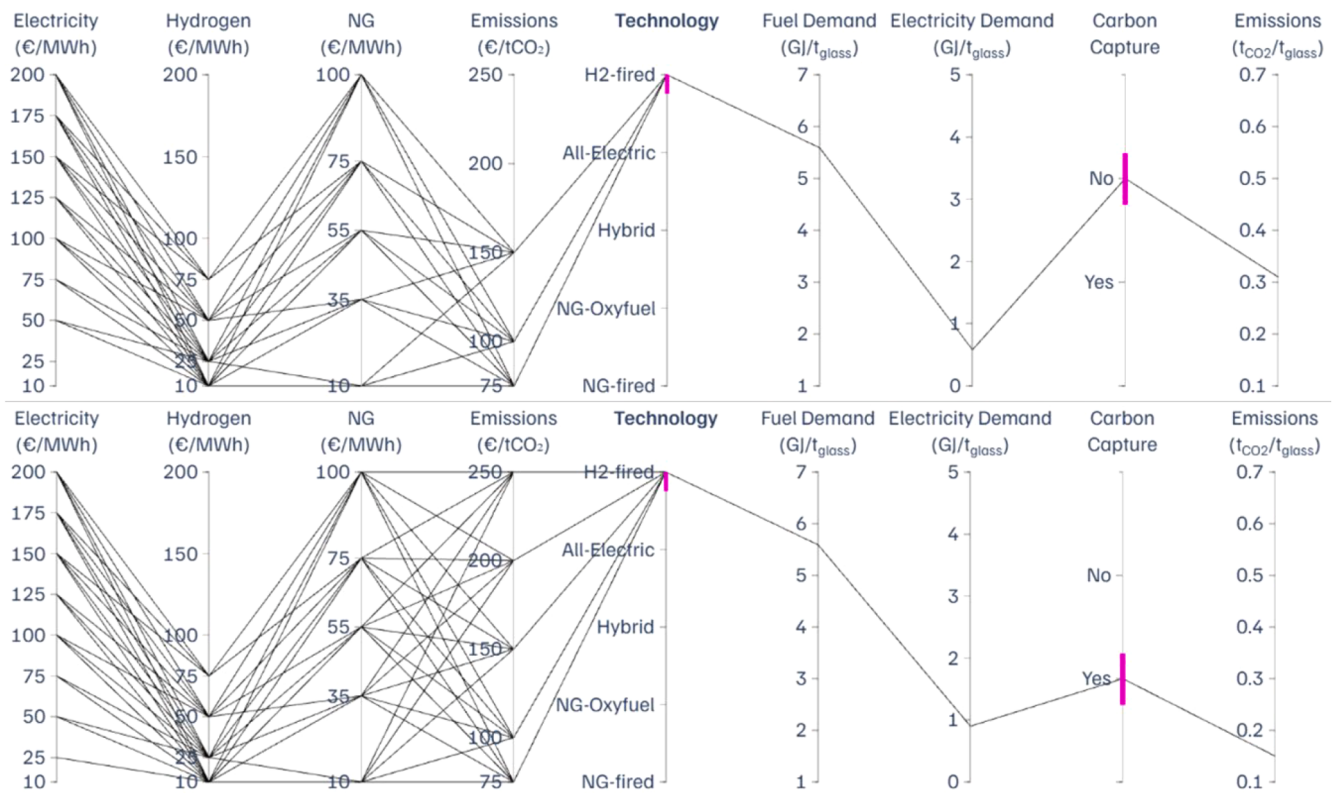
Fig. 15. Parallel coordinates plot depicting solution space of H2fur (top) and H2fur-CC (bottom), as a function of the commodities and CO 2 emissions prices.
