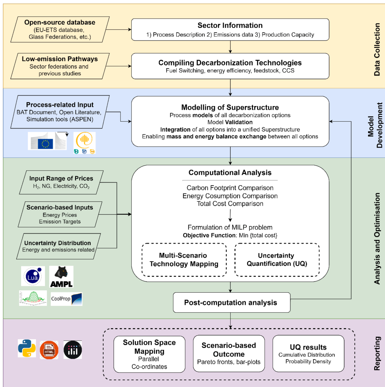
Fig. 1. Comprehensive framework used to design and analyse decarbonisation pathways for glass production.
