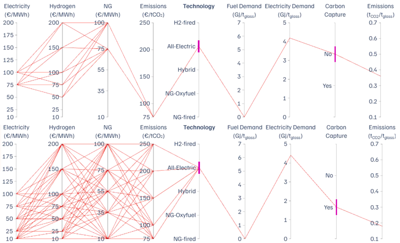
Fig. 14. Parallel coordinates plot depicting solution space of ELfur (top) and ELfur-CC (bottom), as a function of the commodities and CO 2 emissions prices.
