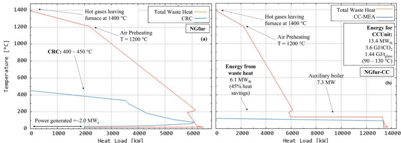
Fig. 4. Integrated composite curves: (a) for NGfur configuration, recovering waste heat via CRC, (b) NGfur-CC configuration, recovering waste heat for CC-MEA unit.
