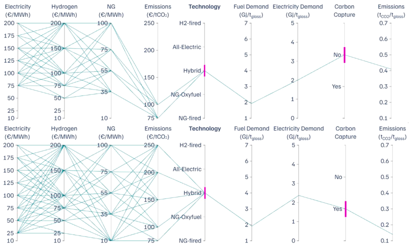
Fig. 13. Parallel coordinates plot depicting solution space of Hybfur (top) and Hybfur-CC (bottom), as a function of the commodities and CO 2 emissions prices.
