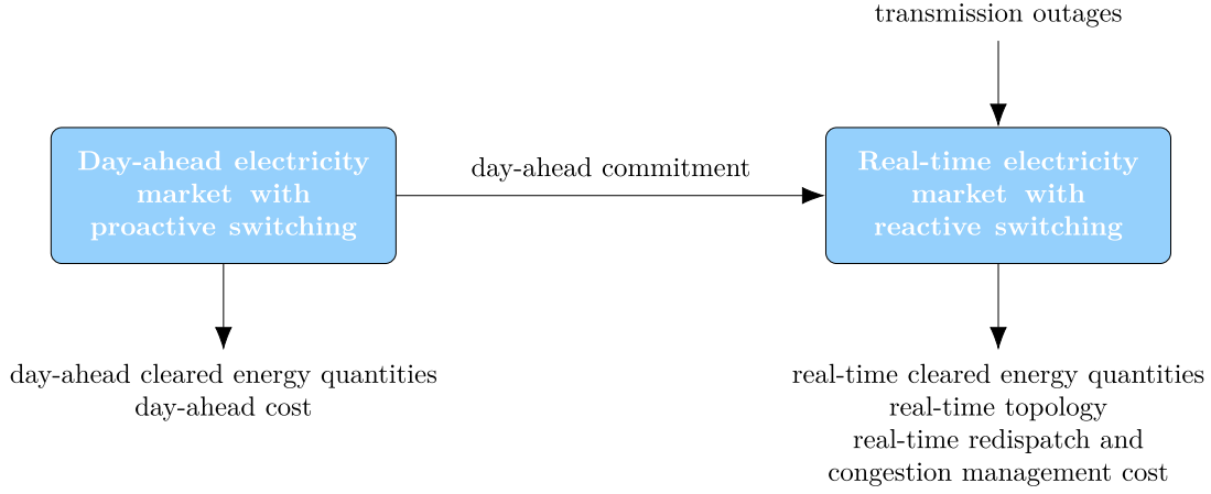
Fig. 2. Block diagram of the two-settlement system used in this work.
