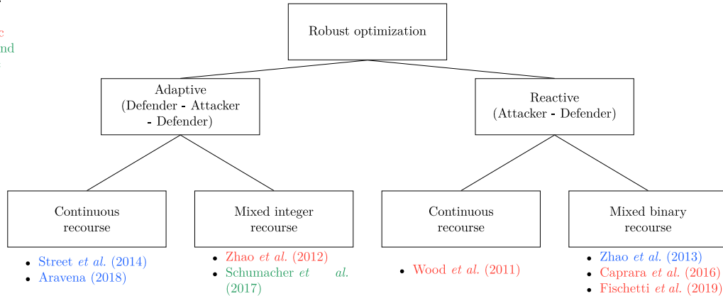
Fig. 1. Decomposition of robust optimization into the different subproblems and the papers associated to each case. We also use a color code to distinguish the modeling and algorithmic contributions.
