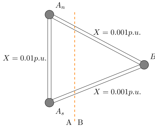
Fig. 3. Network data of the three-node two-zone example that is presented in the appendix.
