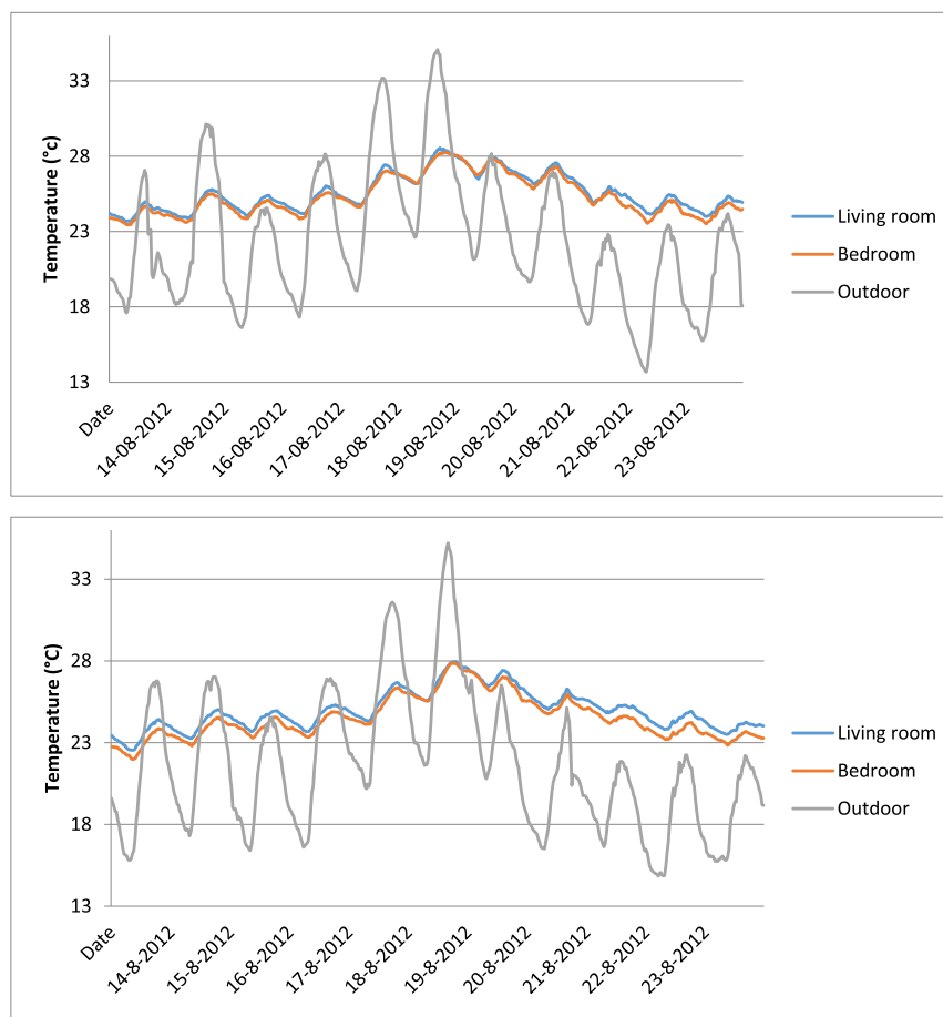
Fig. 1. Variation of half-hourly average temperatures living rooms, bedrooms and outdoor temperature in °C in Arnhem (upper) and Groningen (lower), 14–24 August (mean of all dwellings).
