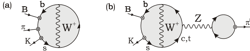
Fig.2 Double-Cabibbo-enhanced B \rightarrow \{\pi K\} decay diagrams:
