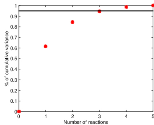
Figure 2: PCA results giving the total variance explained with respect to the number of reactions.
