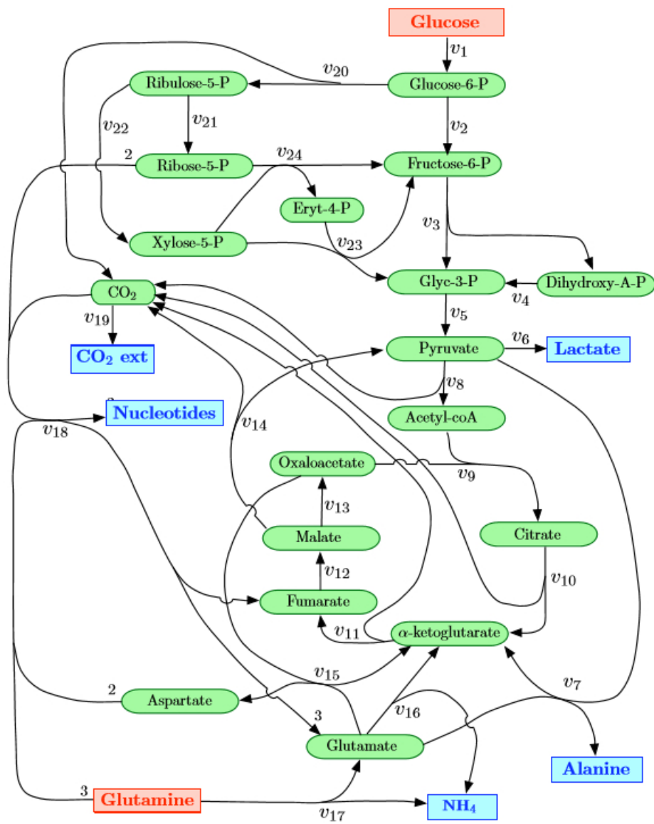
Figure 1: Metabolic network for mammalian cell central metabolism.
