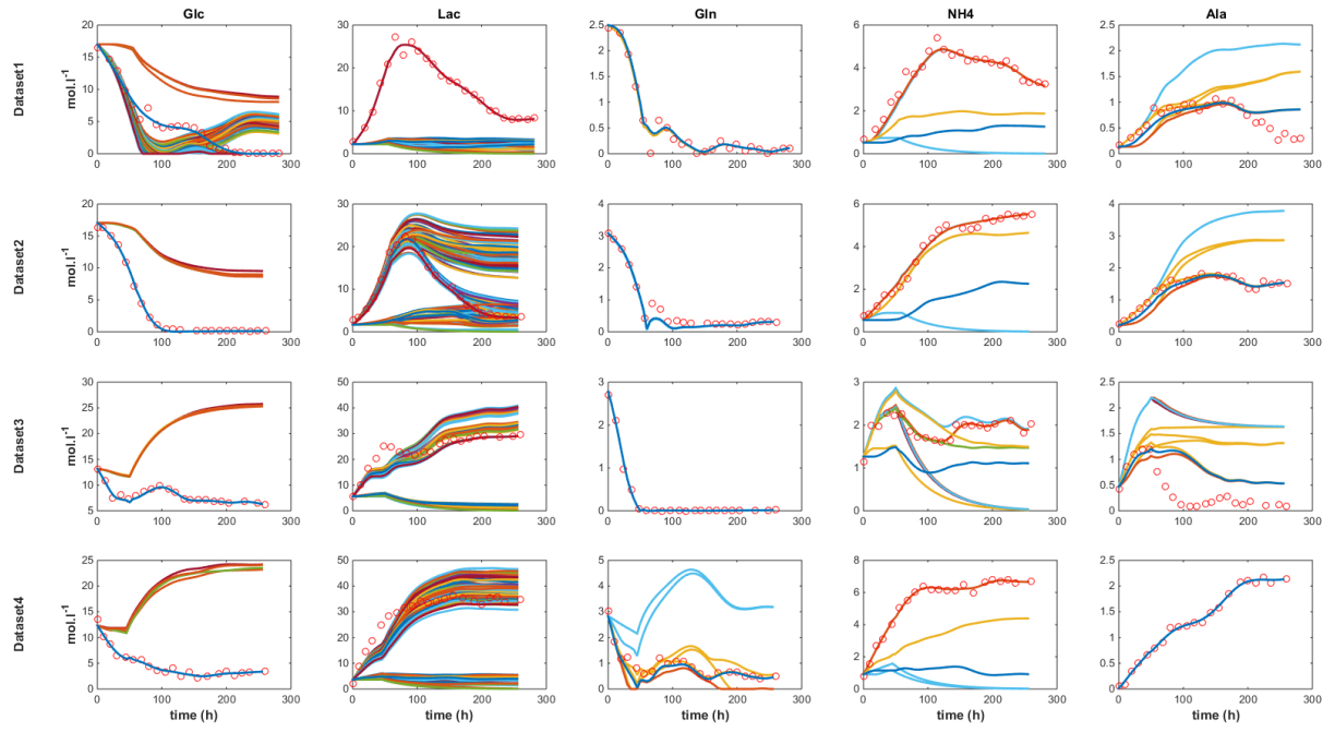
Figure 3: Time evolution of the concentrations obtained by integration of the solutions of LP (7) for all combinations of 5 EFMs covering the whole network.
