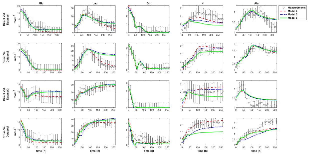
Figure 6: Direct validation of models 4, 5 and 6
