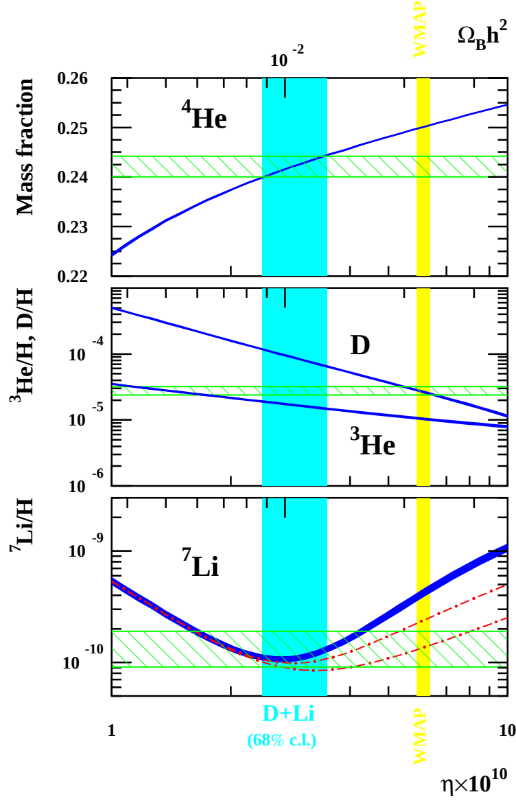
Figure 1. Abundances of ^4\text{He} (mass fraction), \text{D} , ^3\text{He} and ^7\text{Li} (by number relative to \text{H} ) as a function of the baryon over photon ratio \eta or \Omega_b h^2 . Limits ( 1\text{-}\sigma ) are obtained from Monte Carlo calculations. Horizontal lines represent primordial ^4\text{He} , \text{D} and ^7\text{Li} abundances deduced from observational data (see text). The vertical stripes represent the (68% c.l.) \Omega_b h^2 limits provided by WMAP 1 or deduced from ^7\text{Li} and ^4\text{He} observations and SBBN calculations. For the dash-dotted lines in the bottom panel: see text.
