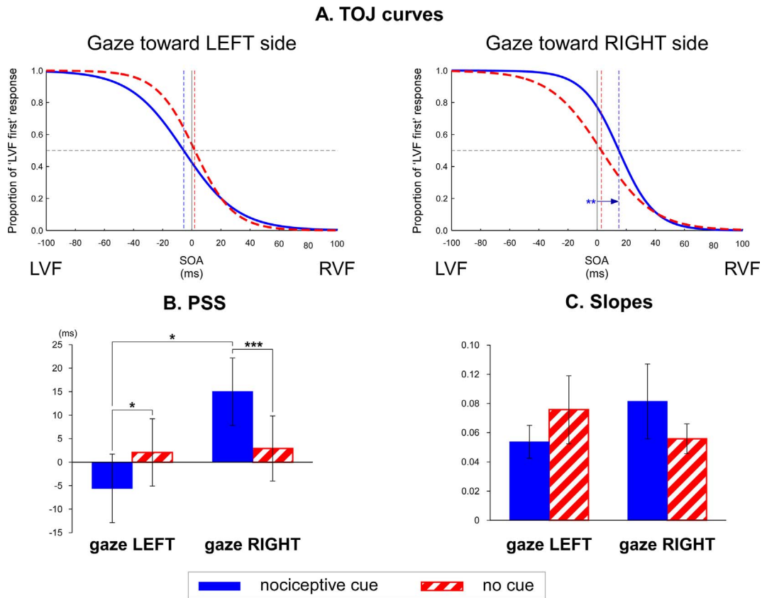
Fig. 2. Averaged results of the 20 participants. The upper part of the figure (A) depicts the fitted logistic functions for the left gaze direction and the right gaze direction conditions. The x-axis represents different hypothetical stimulus onset asynchronies (SOAs) between the two visual stimuli: negative values indicate that the visual stimulus in the left visual hemifield (LVF) was presented first, while positive values indicate that the visual stimulus in the right visual hemifield (RVF) was presented first. The y-axis represents the proportion of trials in which the participants perceived the visual stimulus in the LVF as occurring first. For both left gaze direction and right gaze direction conditions, red dashed curves represent the conditions in which no nociceptive cue was applied on the centrally placed hand, with the corresponding PSS values indicated by the red vertical dashed lines. Blue solid curves represent the conditions in which a nociceptive cue was applied on the hand, with the corresponding PSS values indicated by the blue vertical dashed lines. The blue arrow in the right gaze direction condition indicates the PSS value significantly different from zero. In this condition, when a nociceptive cue was applied, curves are shifted to the RVF, indicating that visual stimuli presented in the RVF had to be presented several ms before the visual stimuli presented in the LVF (i.e. the one spatially congruent with the stimulated hand) to have the chance to be perceived as occurring first equally often. The lower parts of the figure illustrate the mean PSS (B) and slope (C) values, for both the left gaze direction and the right gaze direction conditions. Significant differences are indicated with asterisks (* p \leq .05 , ** p \leq .01 , *** p \leq .001 ). Error bars represent the 95% confidence intervals adapted according to the method of Cousineau (2005). (For interpretation of the references to color in this figure legend, the reader is referred to the web version of this article.)
