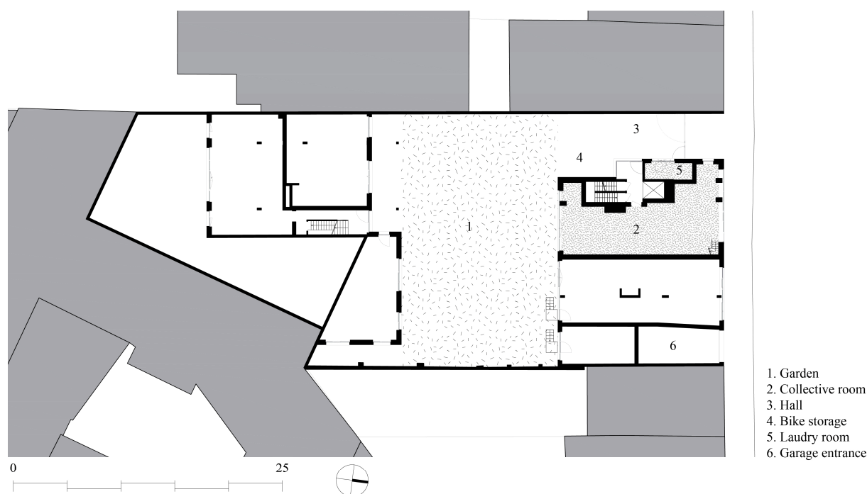
Figure 3. L'Echappée, ground floor—shared spaces (drawn by the authors, 2019).
