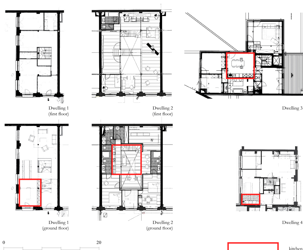
Figure 5. Casa Nova apartments, kitchen position (drawn by the authors, 2019).
