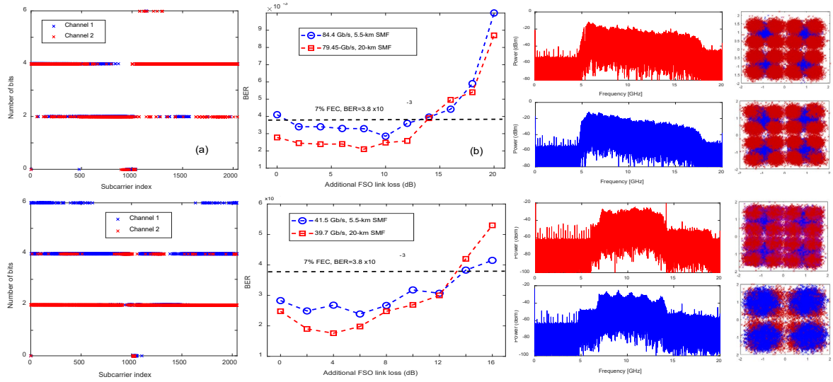
Fig. 3. Performance of 2x2 MIMO signal transmission over the seamless fiber-FSO system in the DL (upper) and UL.
