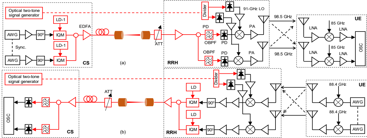
Fig. 2. Experimental setup for 2×2 MIMO mmWave signal transmission over seamless fiber-FSO system: (a) DL, (b) UL.
