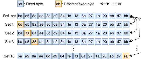
Fig. 1: Illustration of the one-hot TVLA.
