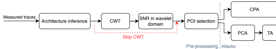
Fig. 5: General attack strategy.
