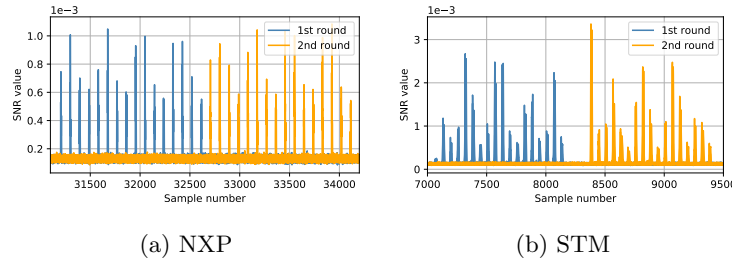
Fig. 3: SNR on first and second rounds for both devices
