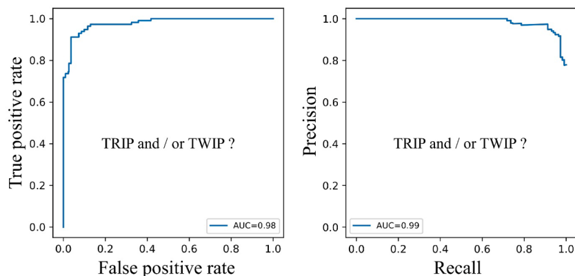
Fig. 5. Receiver Operating Characteristic (ROC) and Precision-Recall curves for the binary prediction ( \beta -metastable or not). Curves are computed over a 5-repeated 5-fold. The Area Under the Curve (AUC) is also given, with higher values corresponding to better performance.
