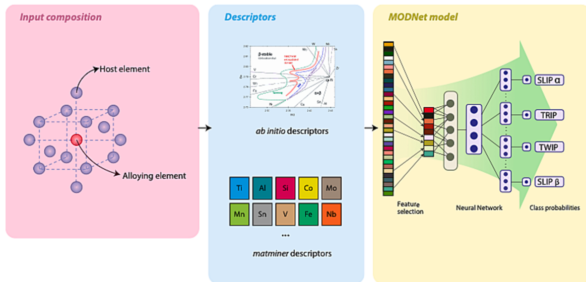
Fig. 2. Methodology for plasticity mechanism prediction. The design procedure consists of constructing a mixed database of calculated and experimental descriptors. MODNet model [30] is then applied to explore the compositional space of Ti alloys. The model returns the probability of activation for each plasticity mechanism as output.
