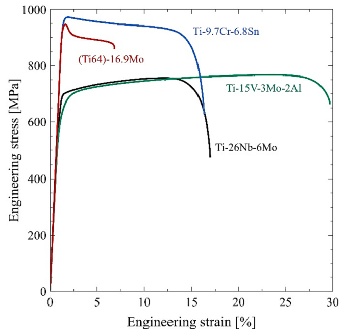
Fig. 6. Engineering stress - strain curves of the new investigated alloys.
