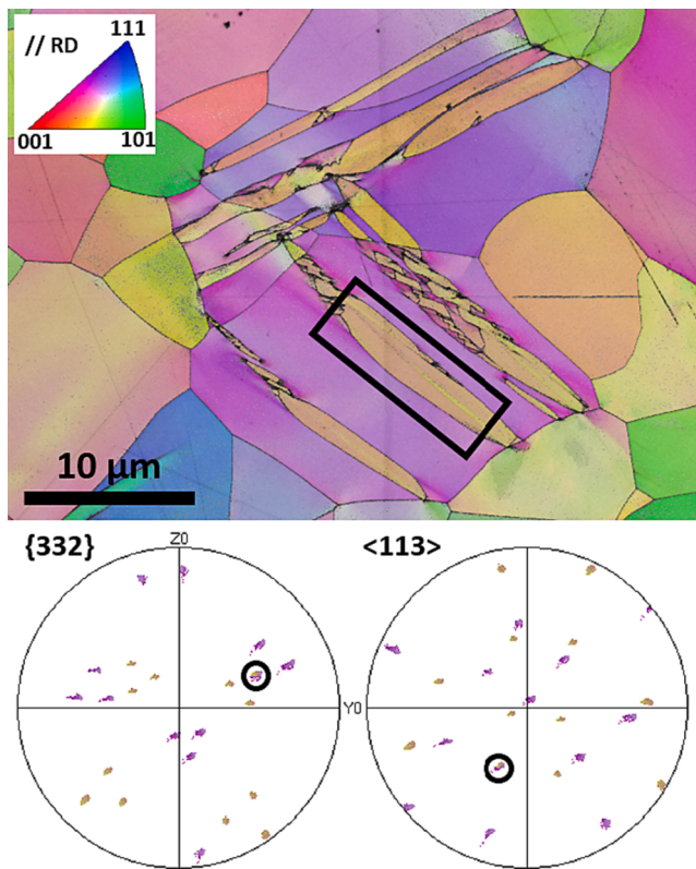
Fig. 8. Inverse pole figure of Ti-26Nb-6Mo alloy strained up to 5 % illustrating the presence of deformation bands. Associated pole figures highlight the {332} <113> twinning relationship of the deformation band present in the black rectangle.
