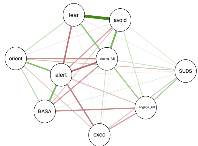
Fig. 1. Association network.
