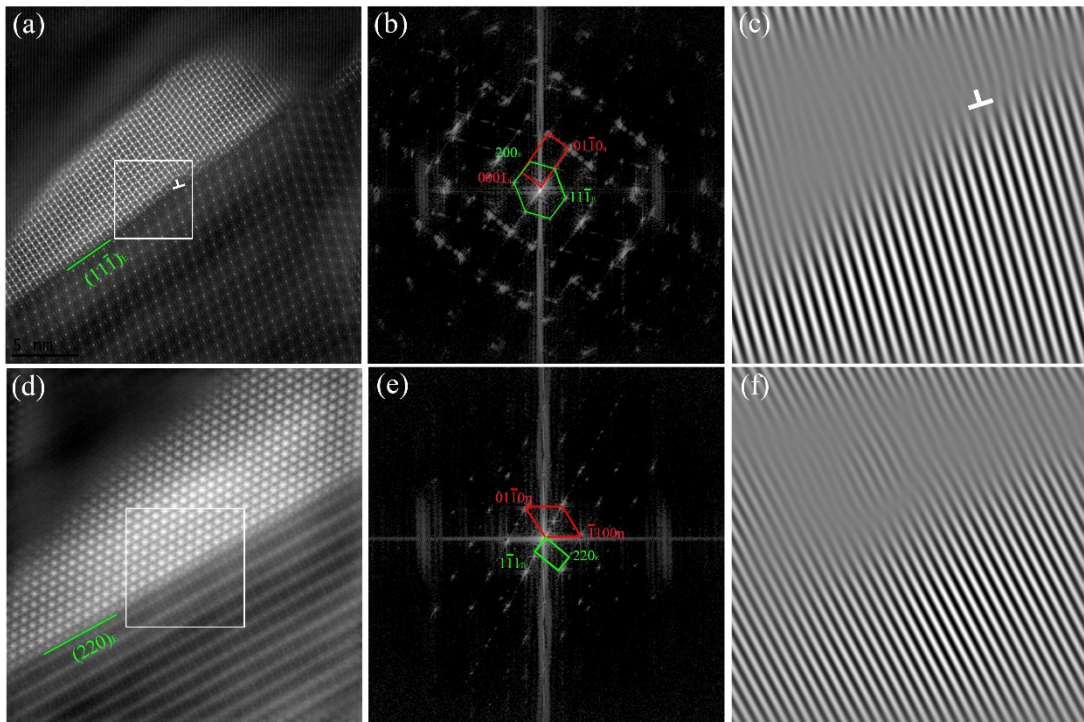
Fig. 9 (a, d) HAADF-STEM images and (b, e) corresponding FFT patterns of the two E/ \eta interfaces. (c and f) show the IFFT image of the (1\bar{1}1)_E planes of the two interfaces.
