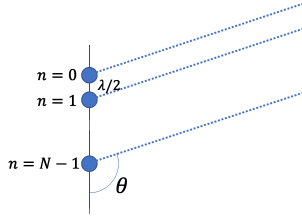
Fig. 1. Array geometry where antennas are separated by \lambda/2 meters.
