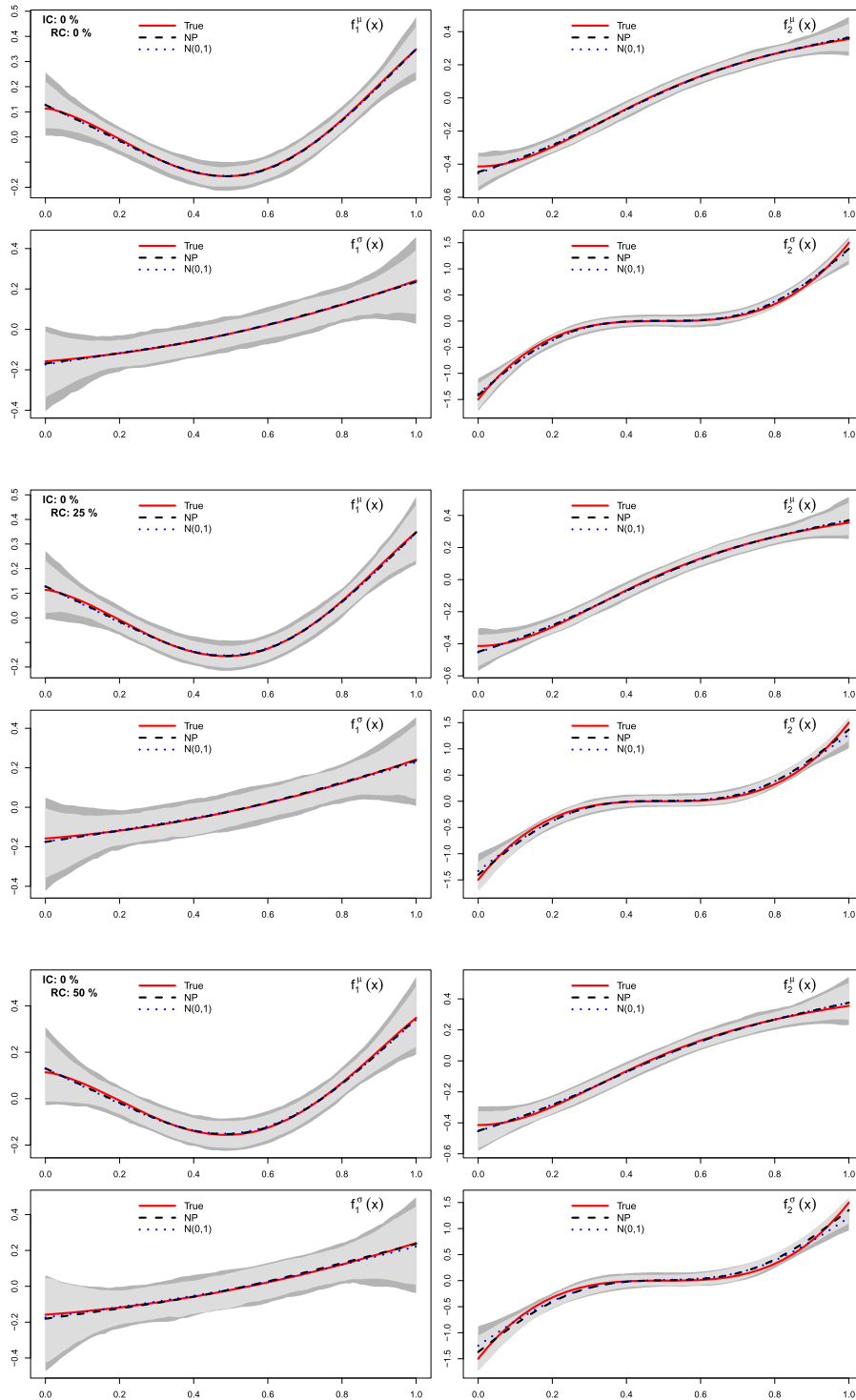
Fig. B.6. Simulation study ( n = 500 ): averaged estimated additive terms (over S = 500 replicates) in the absence of interval-censoring, but for increasing right-censoring rates and by assuming a NP (dashed line) or a Normal (dotted line) error term. Envelopes (light grey: NP; dark grey: Normal) result from consecutive intervals containing 95% of the S estimates for f_j^\mu(x) or f_j^\sigma(x) with x in (0, 1) .
