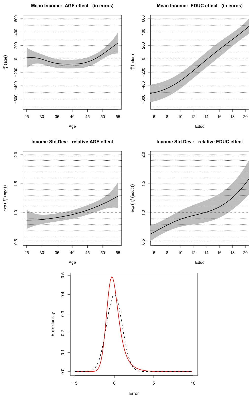
Fig. 1. Belgian income data (ESS 2016): estimated additive terms in the NP-DALSM model with pointwise 95% credible intervals; Row 1 (effects on location): f_1^\mu(\text{Age}) and f_2^\mu(\text{Educ}) rescaled in euros; Row 2 (relative effects on dispersion): \exp(f_1^\sigma(\text{Age})) and \exp(f_2^\sigma(\text{Educ})) ; Row 3: Estimated error density (solid line) compared to the standard Normal (dashed line).
