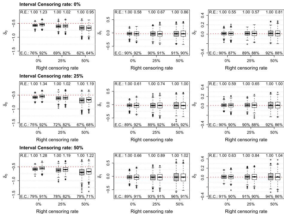
Fig. B.5. Simulation study ( n = 250 ): estimation of the regression parameters in the DALSM model over S = 500 replicates: boxplot of the point estimates under a nonparametric (grey) or Normal (white) error term, Relative Efficiency (R.E.) under the working Normality hypothesis, Effective Coverage (E.C.) of 95% credible intervals.
