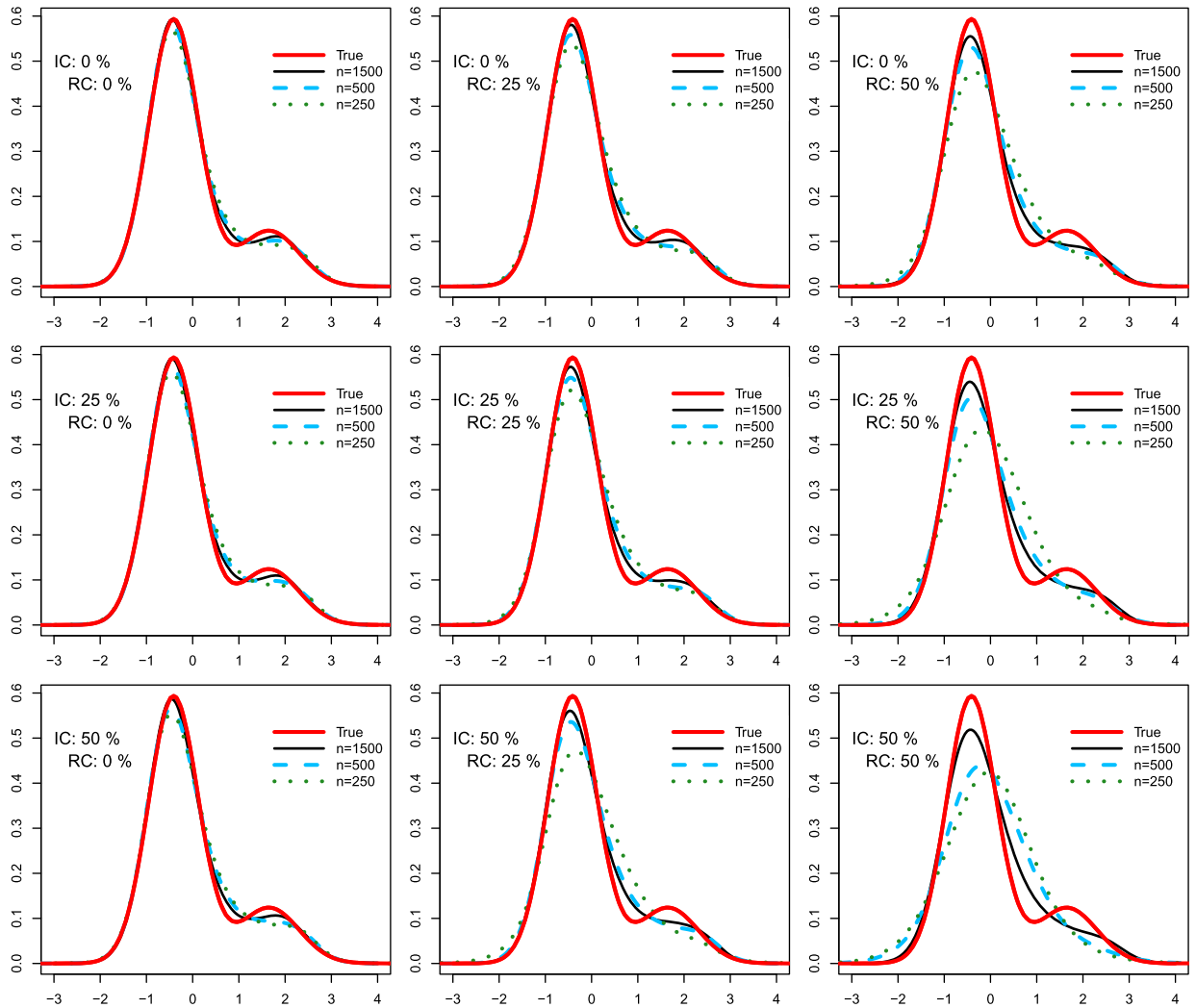
Fig. B.8. Simulation study: estimated error densities in the NP-DALSM model (averaged over the S = 500 replicates) using a NP error term for different combinations of sample sizes, right- (RC) and interval-censoring (IC) rates.
