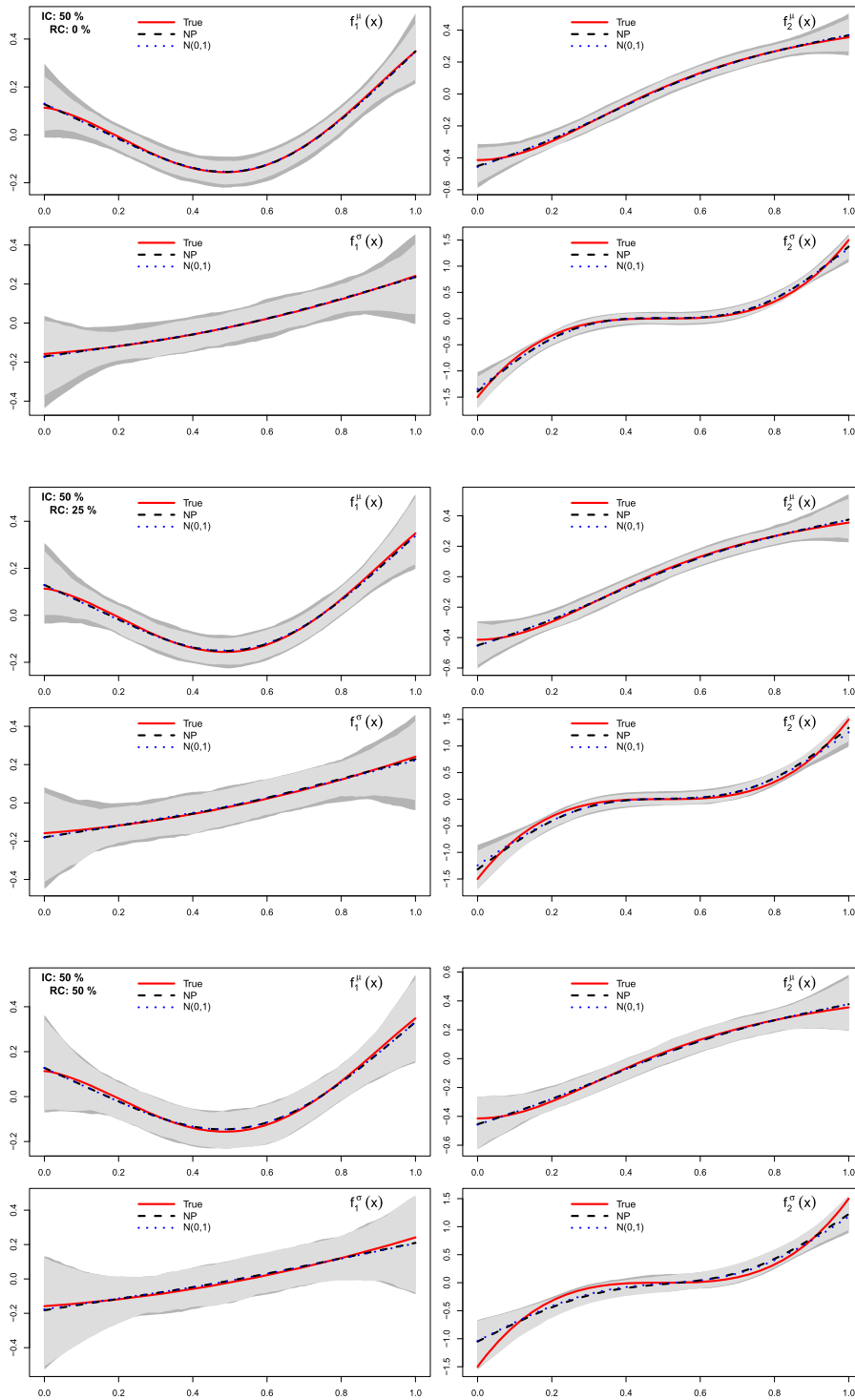
Fig. B.7. Simulation study ( n = 500 ): averaged estimated additive terms (over S = 500 replicates) under a 50% interval-censoring rate combined with increasing right-censoring rates and by assuming a NP (dashed line) or a Normal (dotted line) error term. Envelopes (light grey: NP; dark grey: Normal) result from consecutive intervals containing 95% of the S estimates for f_{f_j^\mu}(x) or f_{f_j^\sigma}(x) with x in (0, 1) .
