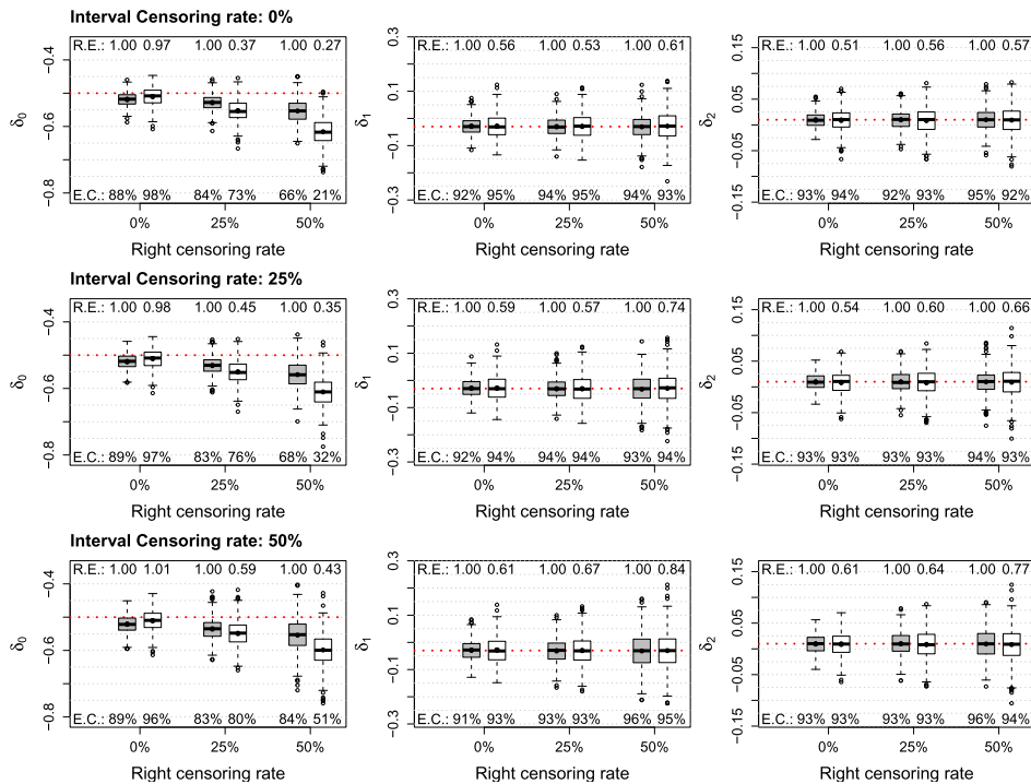
Fig. B.3. Simulation study ( n = 1500 ): estimation of the regression parameters in the DALSM model over S = 500 replicates: boxplot of the point estimates under a nonparametric (grey) or Normal (white) error term, Relative Efficiency (R.E.) under the working Normality hypothesis, Effective Coverage (E.C.) of 95% credible intervals.
