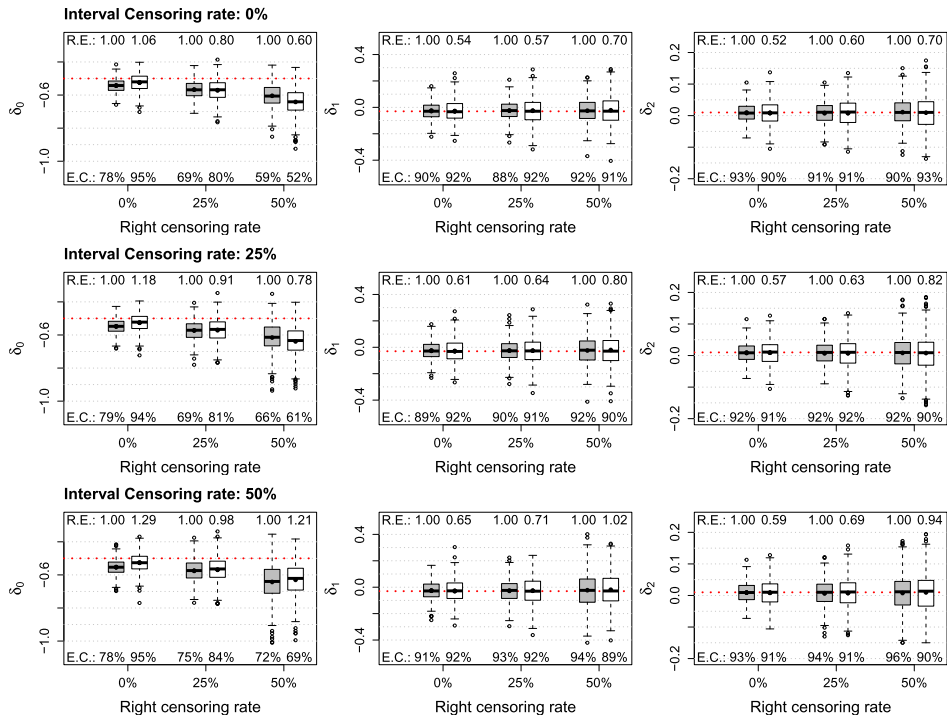
Fig. B.4. Simulation study ( n = 500 ): estimation of the regression parameters in the DALSM model over S = 500 replicates: boxplot of the point estimates under a nonparametric (grey) or Normal (white) error term, Relative Efficiency (R.E.) under the working Normality hypothesis, Effective Coverage (E.C.) of 95% credible intervals.
