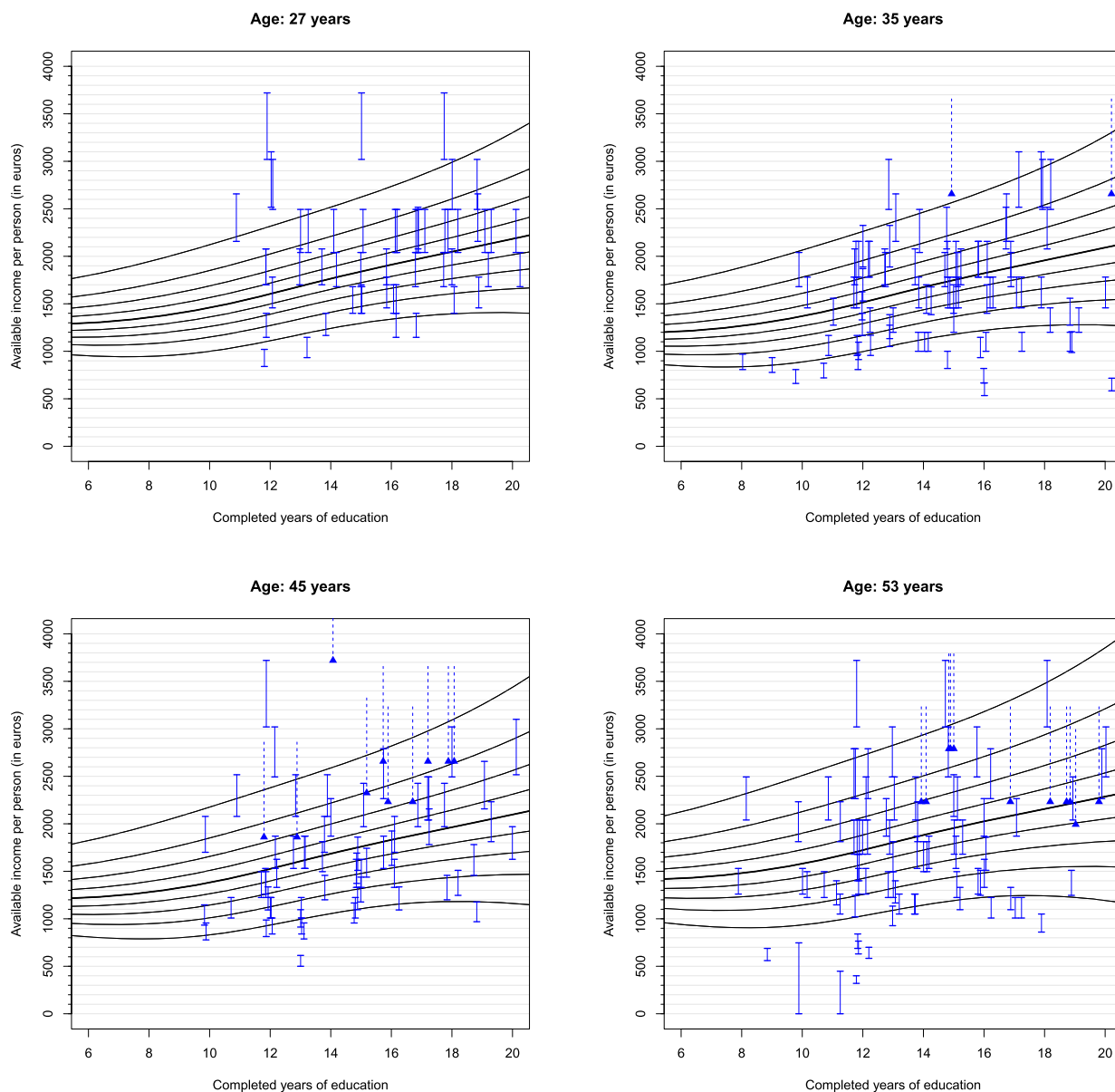
Fig. 2. Belgian income data (ESS 2016): fitted conditional deciles (rescaled in euros) for the income per person in two-income households.
