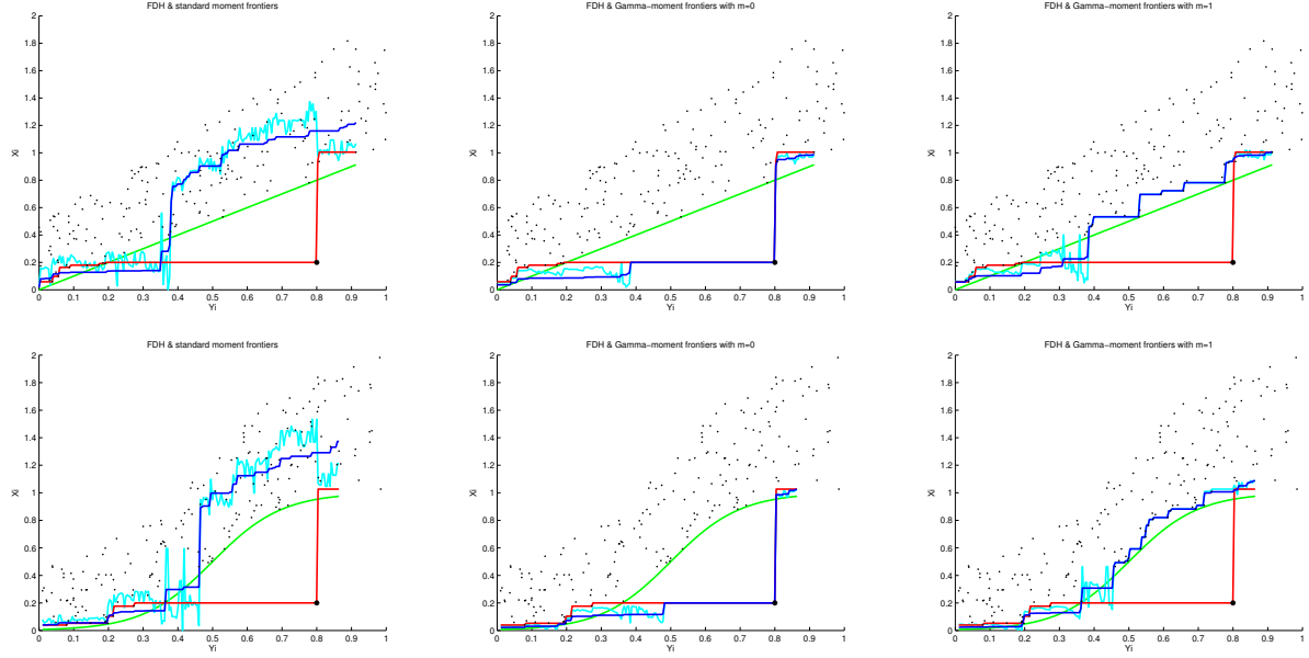
Figure 3: Results for \gamma_y = -1/2 and n = 201 (as in Figure 1 with one outlier included)
