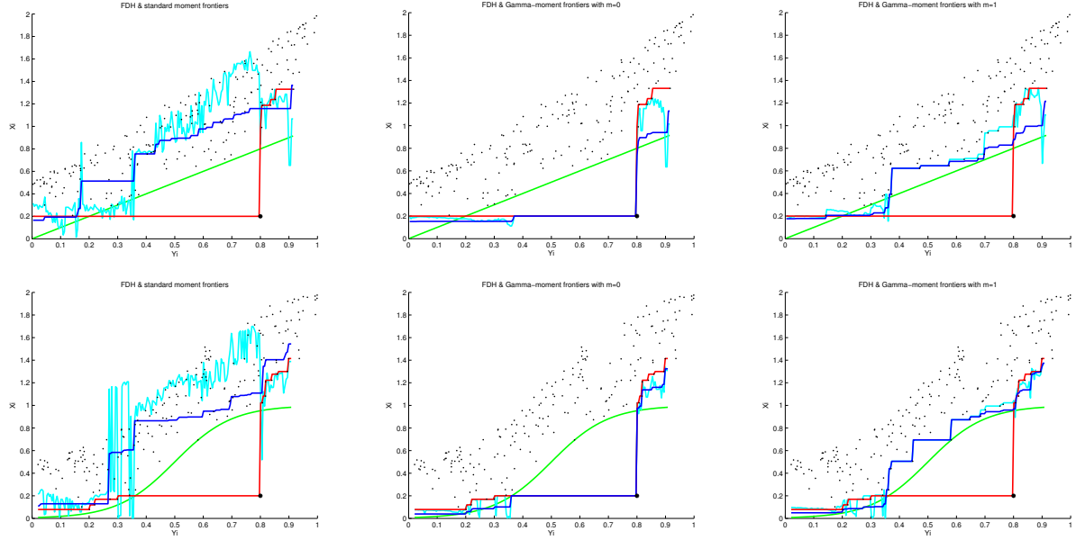
Figure 4: Results for \gamma_y > -1/2 and n = 201 (as in Figure 2 with one outlier included).
