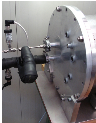
Figure 3.26: The lid of the vacuum vessel.
