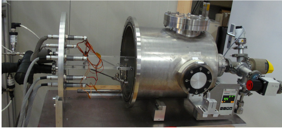
Figure 3.25: The vacuum vessel fully equipped before closing.
