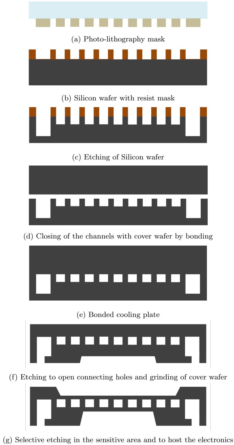
Figure 3.18: Simplified production process of a micro channel heat sink.
