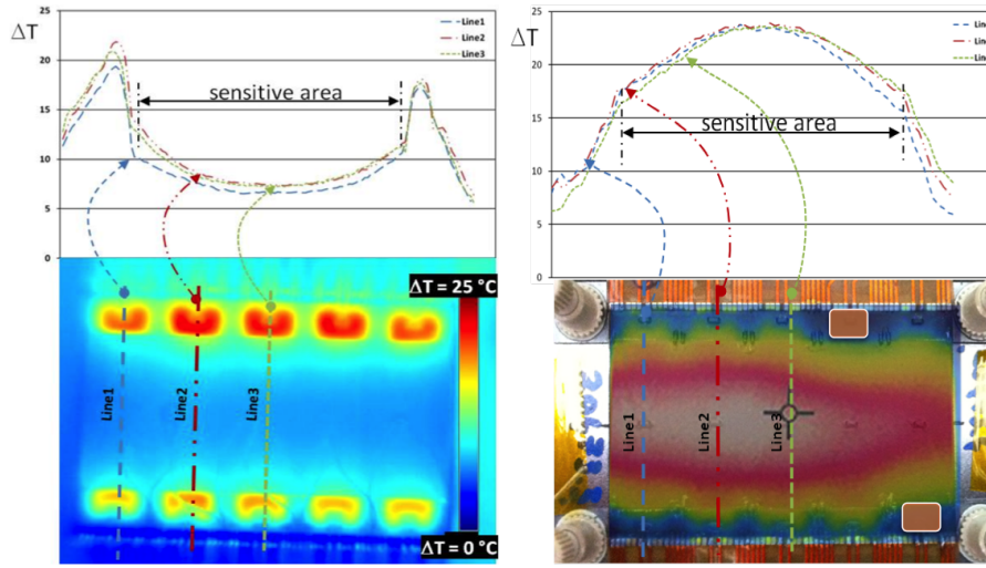
Figure 4.27: Cooling plate and cooling frame with temperature lines over their surface.
