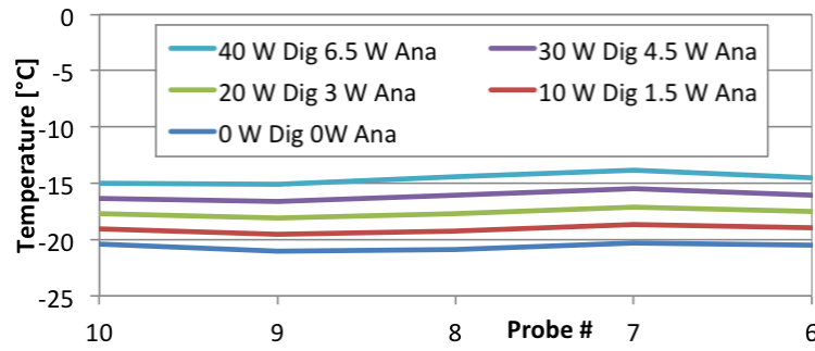
Figure 4.10: Temperatures of the analogue part for different power settings.
