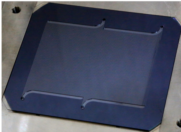
Figure 5.5: Baseline micro channel cooling plate.
