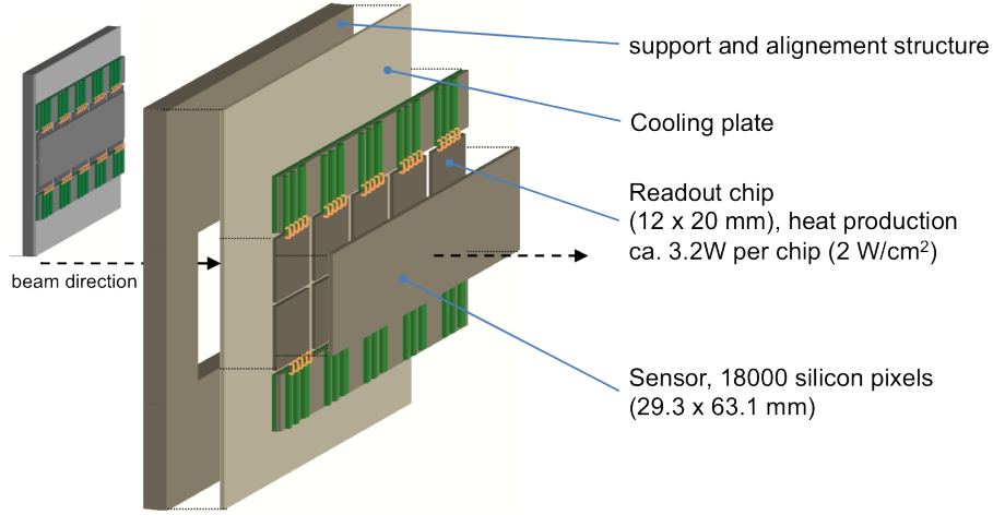
Figure 1.5: Schematic view of one GTK module
