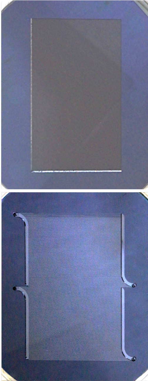
Figure 3.7: Baseline cooling plate with double inlet/outlet, backside with impression to host the readout chips/dummy electronics.
