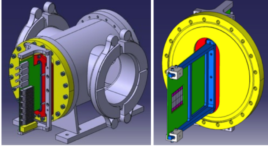
Figure 5.1: GTK housing with installed GTK module and inside view. Courtesy of Nicolas Szilasi, UCL, Belgium
