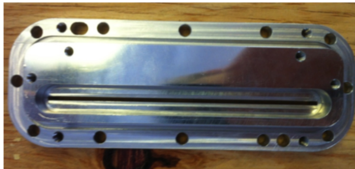
Figure 5.7: Flange for repeatable geometrical precision during installation.
