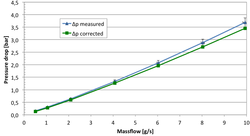
Figure 4.14: Measured pressure drop of the alternative cooling frame at -20 °C fluid inlet temperature. The error bars on the measured values are magnified 10 times to make them visible.
