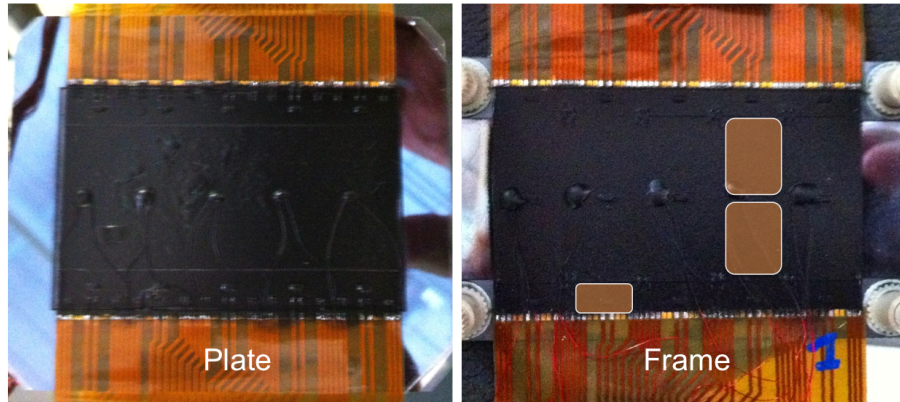
Figure 4.22: Baseline cooling plate and alternative cooling frame with black painted silicon mock-ups.
