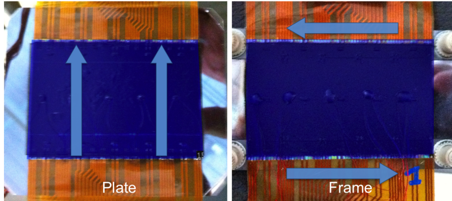
Figure 4.24: Cooling plate and cooling frame without power on silicon mock-ups. Coolant runs with 15 °C inlet temperature.
