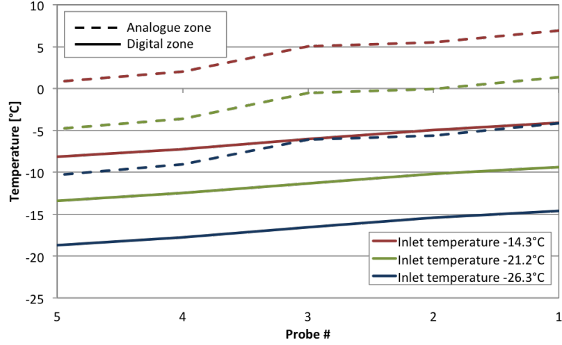
Figure 4.20: Measured temperature of the analogue zone and approximated temperature of on digital zone with quasi nominal power settings at different inlet temperatures.
