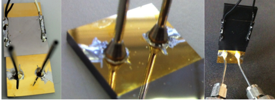
Figure 5.15: Two tubes soldered on to a mc heat exchanger for ATLAS inner detector.
