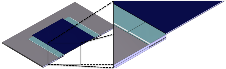
Figure 3.12: Cross section of the cooling frame in real dimensions. Enlargement of EoC region with micro channels running underneath.
