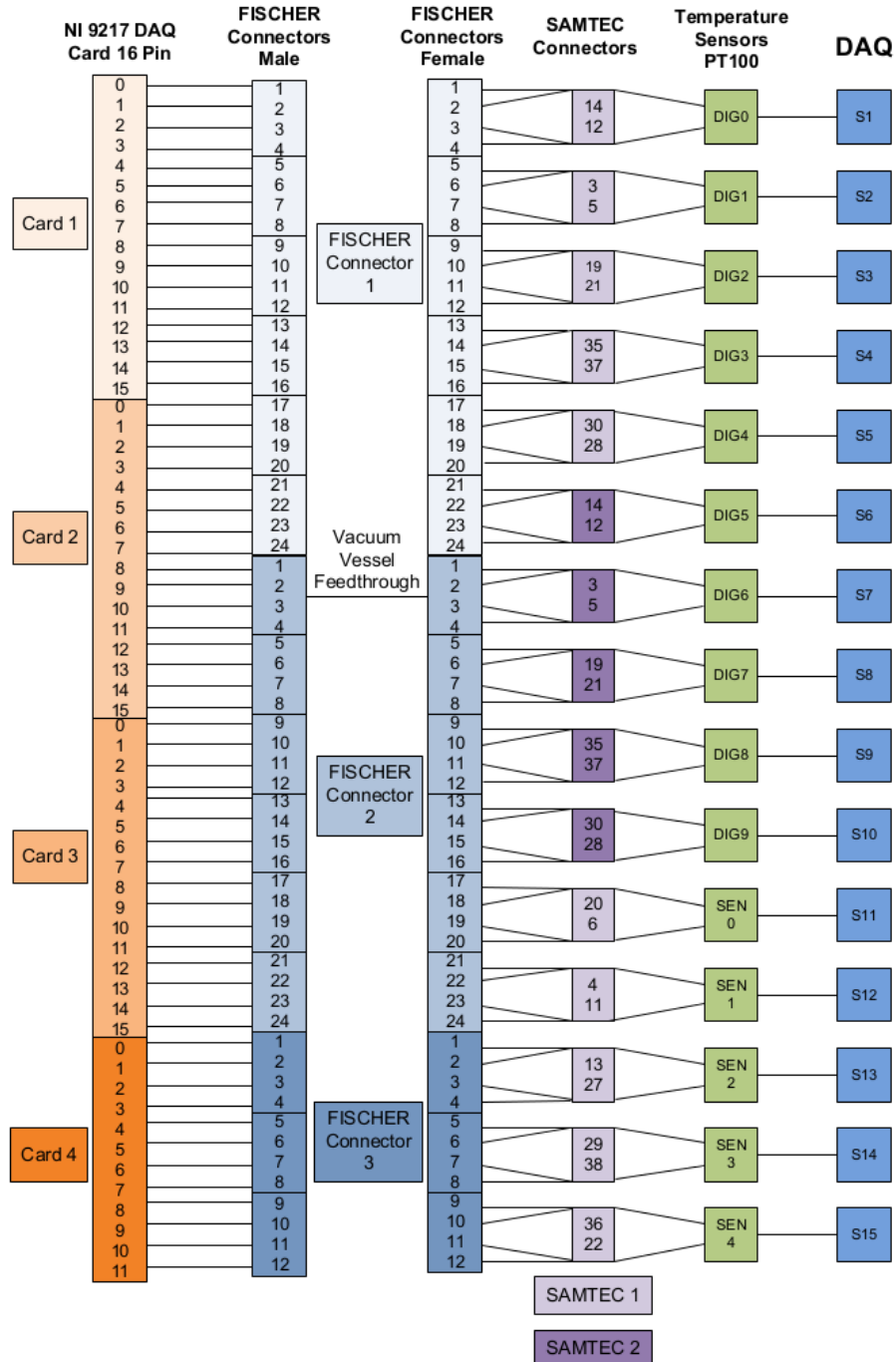
Figure 6.3: Wiring scheme for the electronics mock-up.
