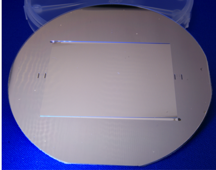
Figure 3.5: Silicon micro channel wafer with pyrex cover, deep manifolds and inlet/outlet diagonally opposite to each other
