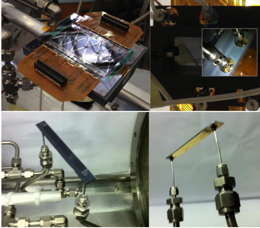
Figure 5.18: Plate and frame stave installed in the mc test stand for hydraulic and thermal test.
