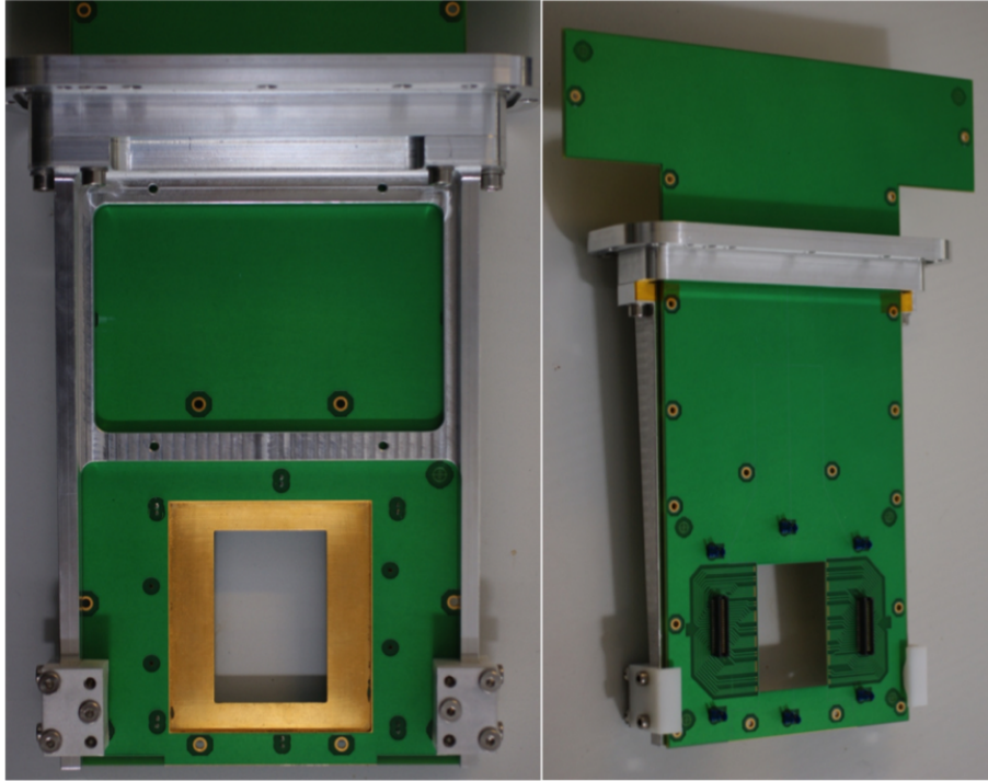
Figure 5.6: Printed circuit board, front and back. Flange and support are mounted for trials.
