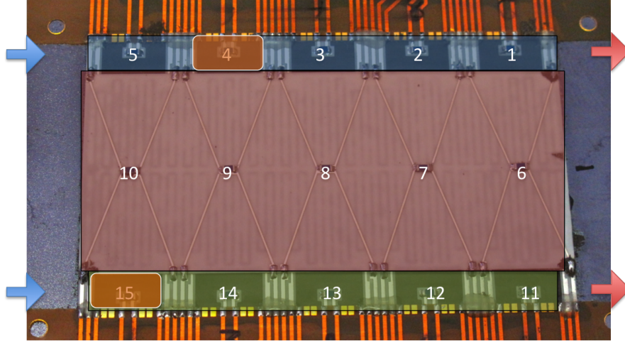
Figure 4.15: Silicon mock-up: numbering of temperature probes, flow direction and inlet/outlet (blue/red arrows) configuration and marking of 2 broken heaters in the digital zones.
