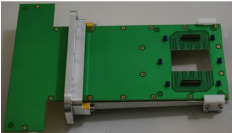
Figure 3.23: PCB for micro channel cooling and assembly tests.
