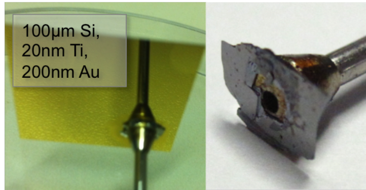
Figure 5.13: A first soldering trial on a 100 \mu\text{m} thick silicon piece. The silicon ruptured at 37 bar water pressure.
