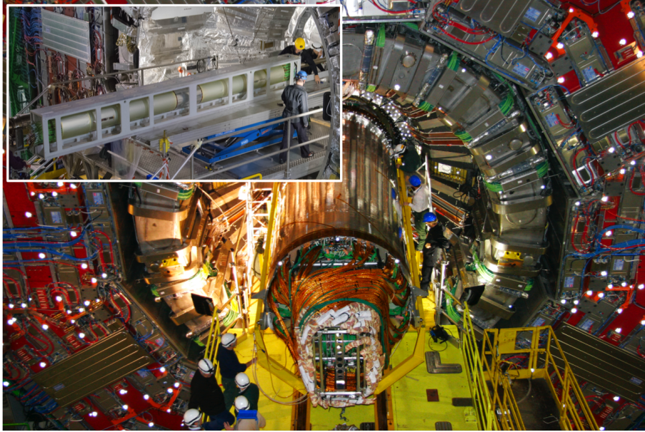
Figure 2.6: The CMS silicon strip tracker (large picture) and the CMS silicon pixel tracker (small picture) before the installation into the experiment. Courtesy of the CMS experiment
