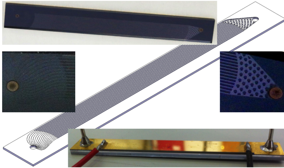
Figure 4.29: Cooling frame stave with micro channels for \text{CO}_2 and solder connectors, see 5.2.1.
