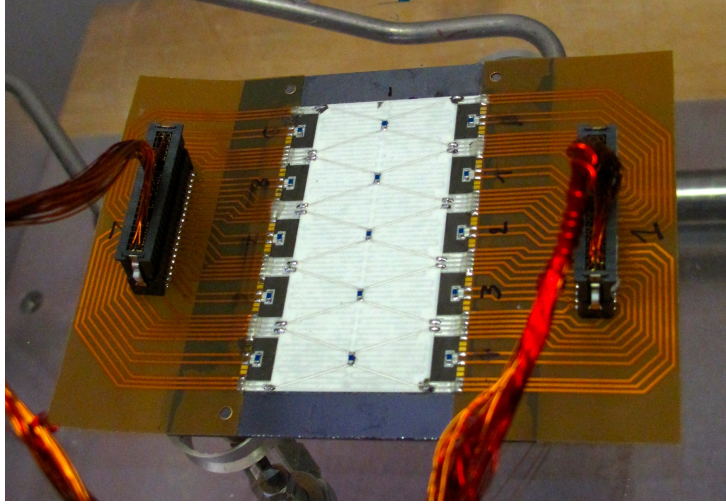
Figure 3.20: Ceramic mock-up glued on baseline mc cooling plate.
