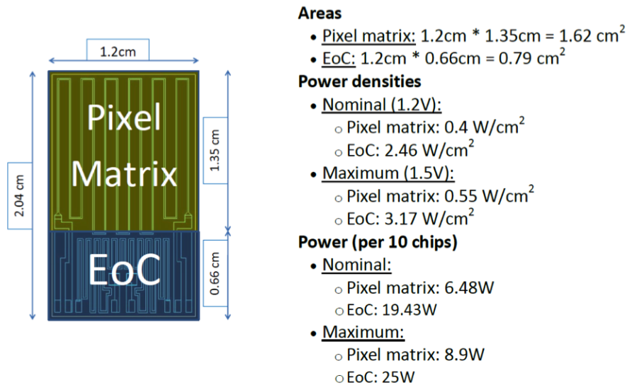
Figure 4.1: Simulated thermal power output of the TDCpix in 2013 and electrical power input into the mock-up electronics.
