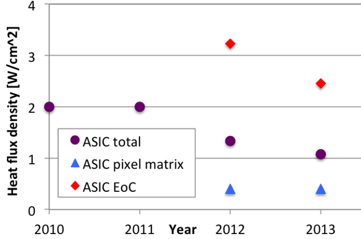
Figure 4.2: Predicted or simulated heat flux density of the TDCpix for nominal power settings over the time of the project.
