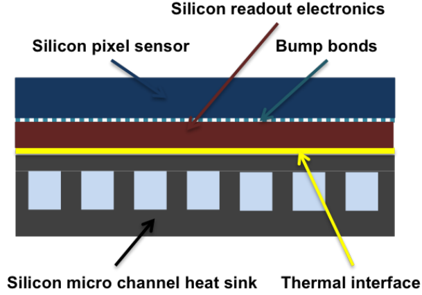
Figure 2.8: Principle of cooling with micro channels
