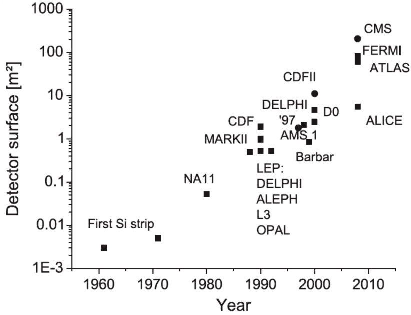
Figure 2.3: The increase of installed active silicon surface over the last decades strikingly proves the importance of silicon detectors in HEP and the rising needs for cooling [42].
