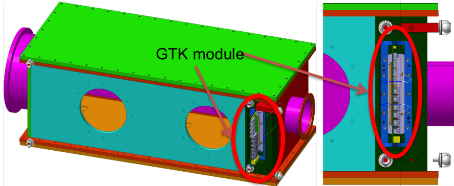
Figure 5.3: GTK module at position 3 integrated into the CHANTI vessel. Courtesy of the CHANTI subdetector group
