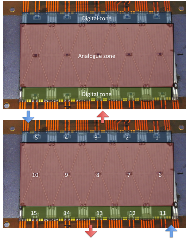
Figure 4.7: Silicon mock-up: zones and numbering of temperature probes and inlet (blue arrow) and outlet (red arrow) configuration.
