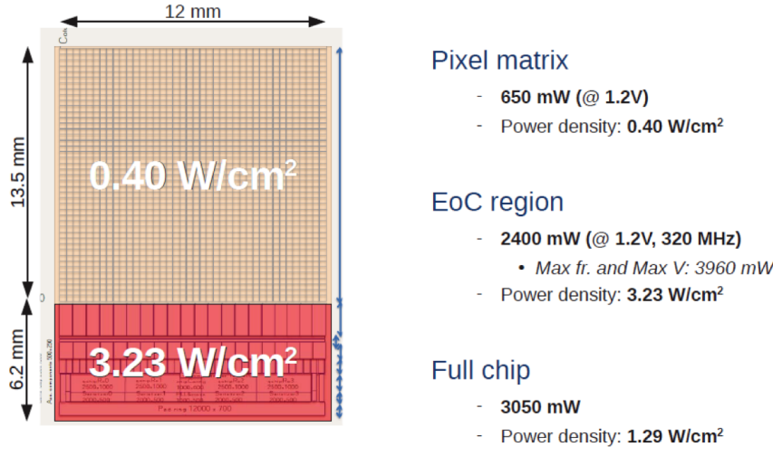
Figure 3.10: Estimated power dissipation of the TDCpix readout chip [67]
