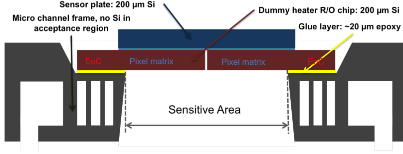
Figure 3.11: Schematic of the cooling frame with electronics.
