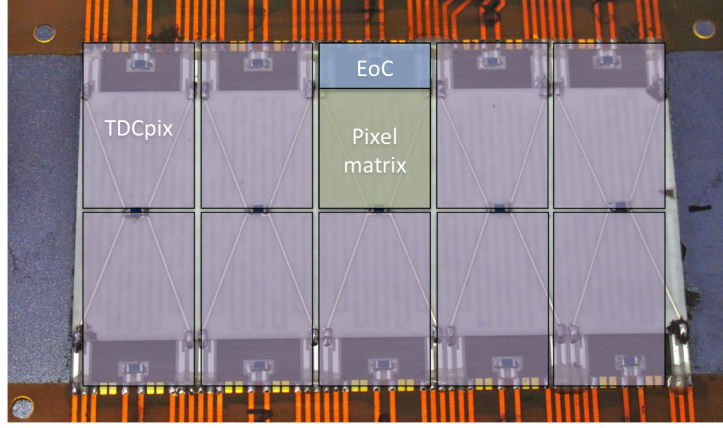
Figure 4.3: Mock-up electronics: configuration of the 10 TDCpix compared to the heaters on the mock-ups.
