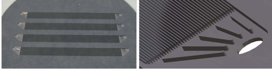
Figure 3.15: Wafer with 4 mc staves in an intermediate production step. 3D drawing of the inlet/outlet region.
