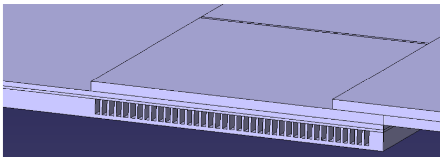
Figure 4.13: 3d Catia model of the cooling frame, the readout chips and the pixel sensor, cut in the center.
