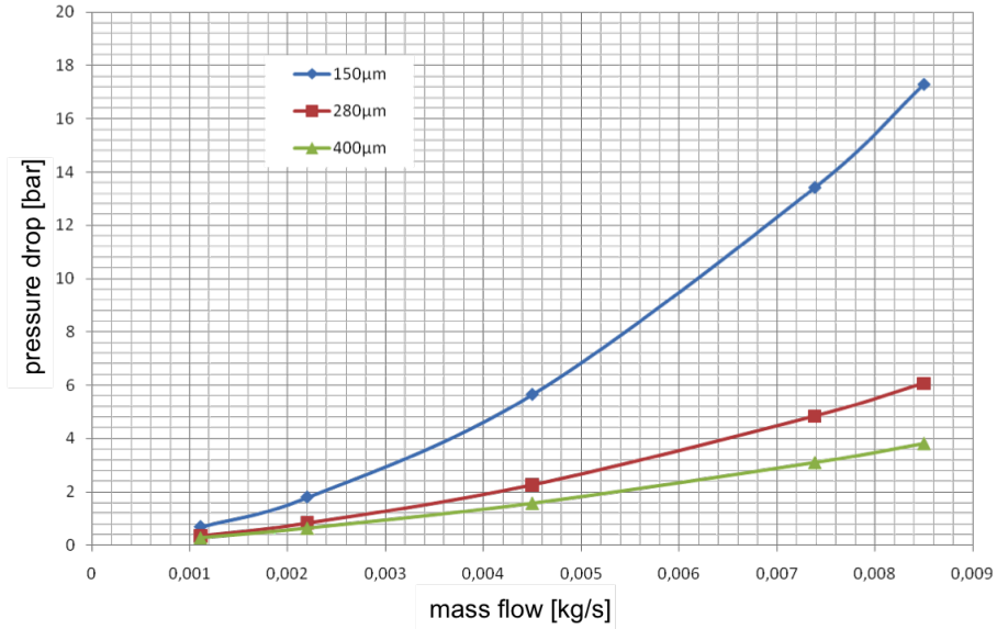
Figure 3.4: Simulated total pressure drop over the mass flow. Manifold depth has a big influence on total pressure drop.
