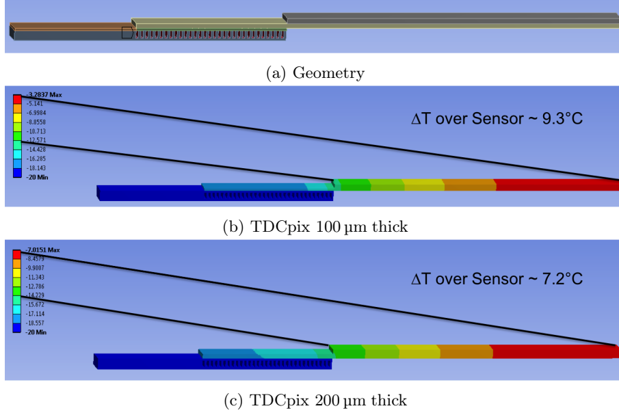
Figure 3.13: Simulation of temperature distribution in a GTK detector mounted on a cooling frame. The wall temperature of the channels is fixed to -20^\circ\text{C} .
