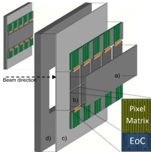
Figure 3.9: Schematic of the GTK subdetector and its readout chip TDCpix.
