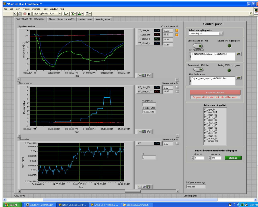
Figure 3.29: DAQ: LabView graphical user interface
