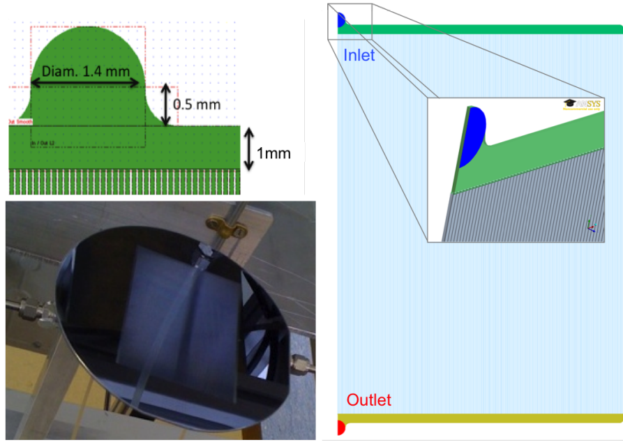
Figure 2.11: First micro channel prototype with central inlet and outlet in hydraulic test; belonging CFD half model.
