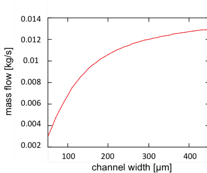
Figure 2.10: Mass flow rate of \text{C}_6\text{F}_{14} over channel width w for the GTK micro channel heat sink ( h = 90\text{ }\mu\text{m} , \Delta p = 2\text{ bar} , b = 3/2 w )
