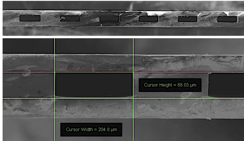
Figure 3.2: Magnification of a cross section cut through a baseline cooling plate, the silicon wafer with channels is fusion bonded to a silicon cover wafer. Courtesy of CSEM
