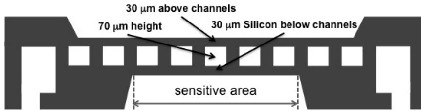
Figure 3.1: Schematic cross section of the baseline design
