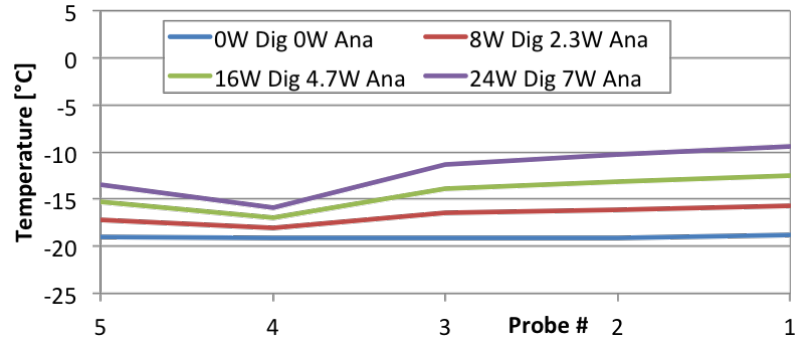
Figure 4.16: Temperatures of the upper digital part for different power settings.
