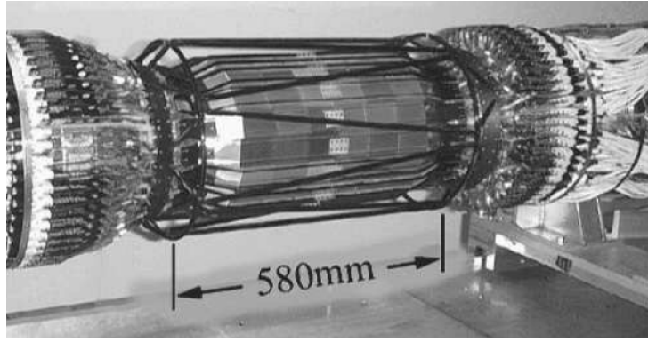
Figure 2.5: The BaBar SVT detector [31]
