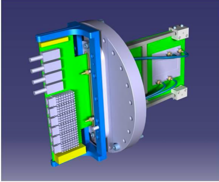
Figure 5.9: The cool assembly inside the PCB, where the TDCpix is wire bonded to the PCB. Courtesy of Nicolas Szilasi, UCL, Belgium
