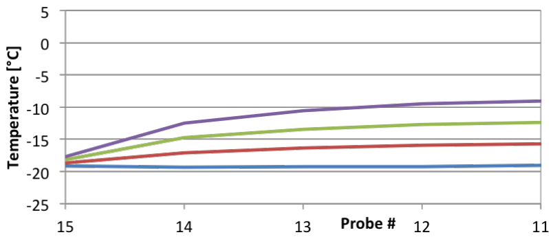
Figure 4.18: Temperatures of the lower digital part for different power settings. (see figure 4.16 for the legend)
