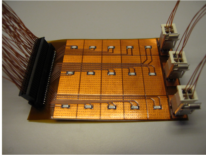
Figure 3.19: The kapton mock-up with 15 PT100 temperature probes and 3 heating zones.
