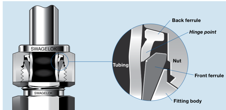
Figure 5.11: The principle of the Swagelok fitting connector [73].
