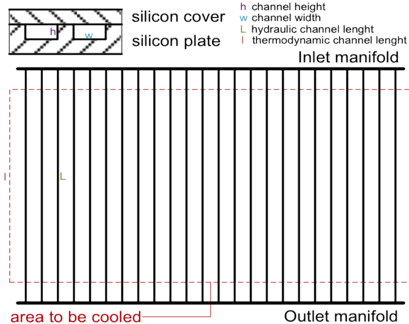
Figure 2.9: Micro channel layout with the important dimensions
