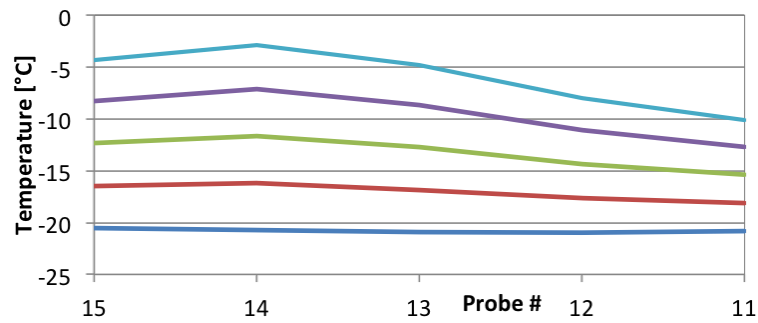
Figure 4.11: Temperatures of the lower digital part for different power settings. (see figure 4.10 for the legend)
