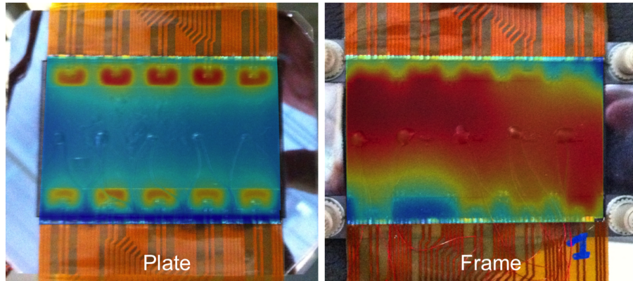
Figure 4.26: Cooling plate and cooling frame with maximal power on silicon mock-ups. Coolant runs with 15 °C inlet temperature.
