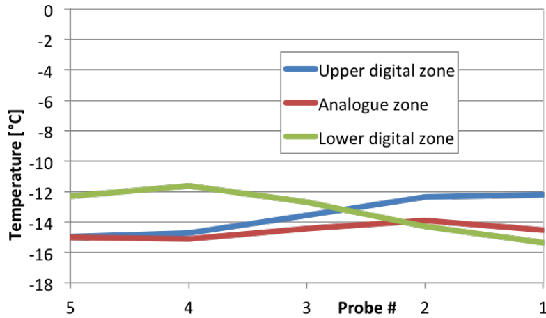
Figure 4.12: Temperatures of silicon mock-up with combined nominal power settings.
