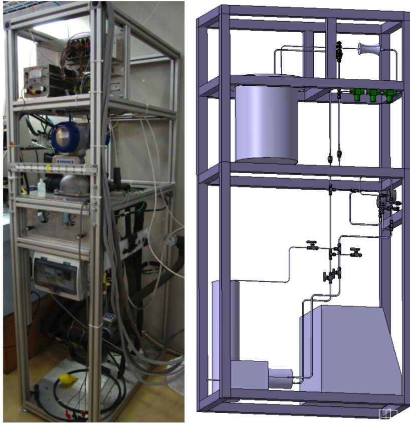
Figure 3.27: Micro channel cooling test rack in the lab and as 3D model
