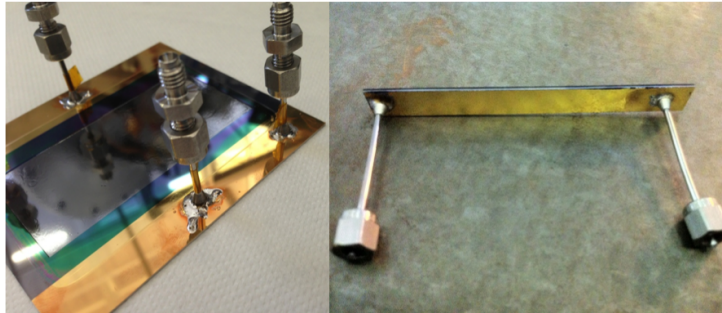
Figure 5.17: GTK baseline cooling plate and cooling frame stave equipped with solder connections.
