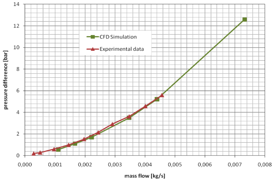
Figure 2.12: Comparison of the measured and the simulated pressure drop of the first prototype.
