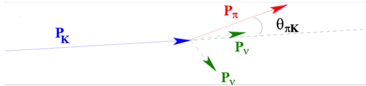
Figure 1.1: Kinematic of the K^+ \rightarrow \pi^+ \nu \bar{\nu} decay
