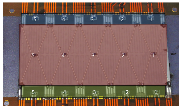
Figure 4.8: Silicon mock-up: alternative numbering of temperature probes, if results from the 2 digital zones and the analogue zone are combined in one graph.
