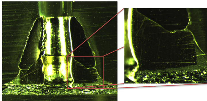
Figure 5.14: Cut of a soldering connection under the microscope. The stainless steel tube is missing, since it was destroyed during the preparation of the cut.
