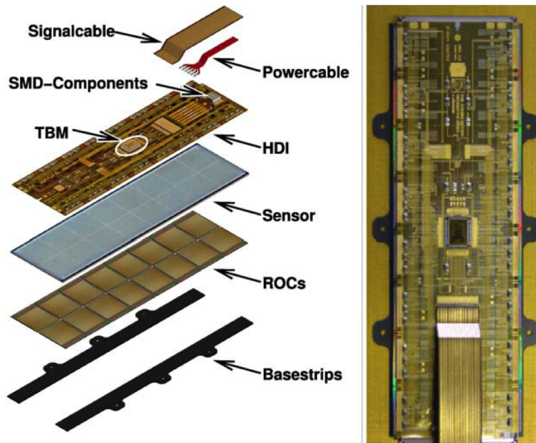
Figure 2.2: A CMS inner tracker pixel module [30].
