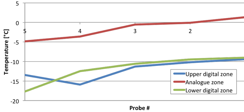
Figure 4.19: Temperatures of silicon mock-up with quasi nominal power settings.
