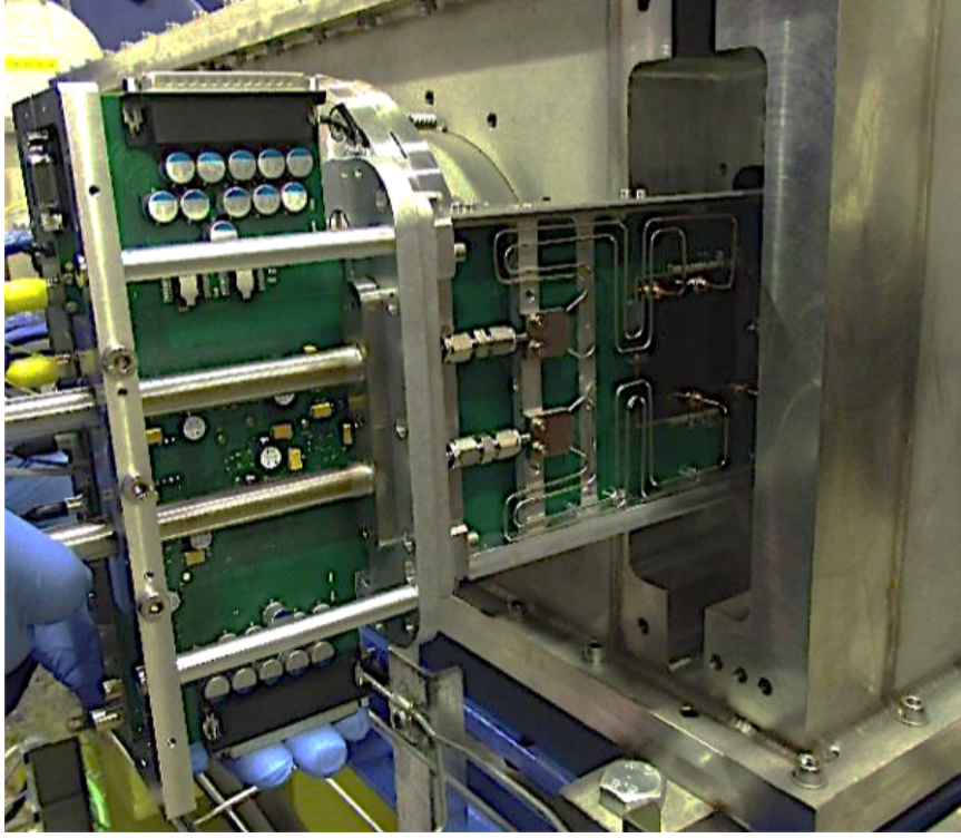
Figure 6.1: The first GTK module before insertion into the vessel on the GTK3-position [28].
