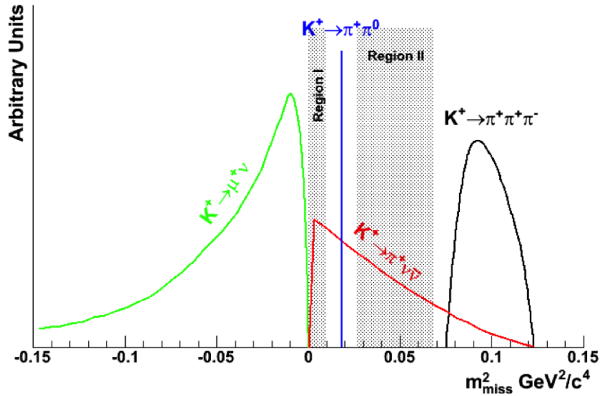
Figure 1.2: Distribution of the missing mass of the K^+ \rightarrow \pi^+ \nu \bar{\nu} decay and dominant background
