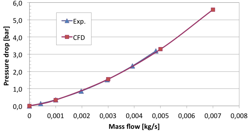
Figure 4.6: Measured and simulated pressure drop of the baseline cooling plate at 15 °C inlet temperature.
