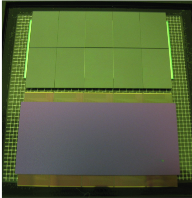
Figure 5.4: Sensor assembly dummy, used to verify the bump bonding process. Courtesy of Massimiliano Fiorini, INFN Ferrara, Italy
