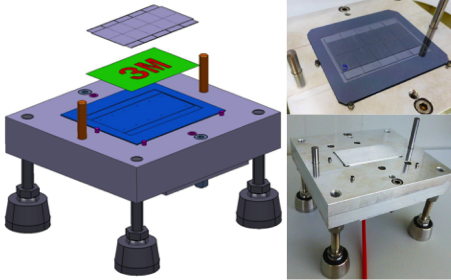
Figure 5.10: The concept of jig 1 includes guiding pins and fixation with vacuum for the different alignment steps. The right side shows a first gluing trial with mechanical dummies. Courtesy of the PH-DT group, CERN, Switzerland
