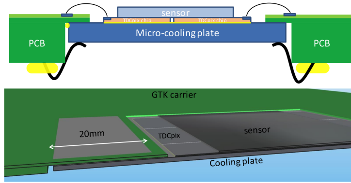
Figure 5.8: The cool assembly inside the PCB, where the TDCpix is wire bonded to the PCB. Courtesy of Michel Morel, CERN, Switzerland
