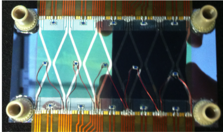
Figure 3.16: Micro channel frame with inlet/outlet connectors and silicon mock-up glued on top. The coolant runs horizontal from left to right or vice versa under the EoC region.
