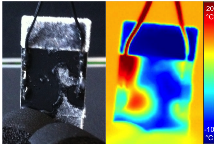
Figure 5.16: Test on a CO 2 cooling plant with an electric power of 36 W.
