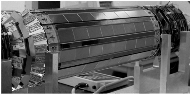
Figure 2.4: The Delphi VTX detector [81]
