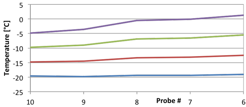
Figure 4.17: Temperatures of the analogue part for different power settings. (see figure 4.16 for the legend)
