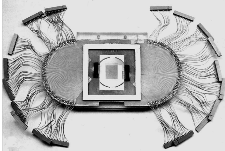
Figure 2.1: A mounted NA11 silicon strip detector [81].
