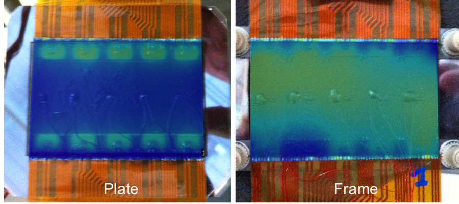
Figure 4.25: Cooling plate and cooling frame with nominal power on silicon mock-ups. Coolant runs with 15 °C inlet temperature.
