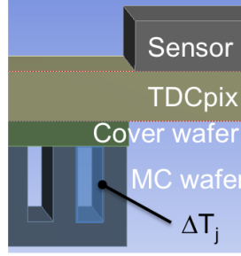
Figure 3.14: Enlarged slice of EoC region to illustrate where \Delta T_j appears.
