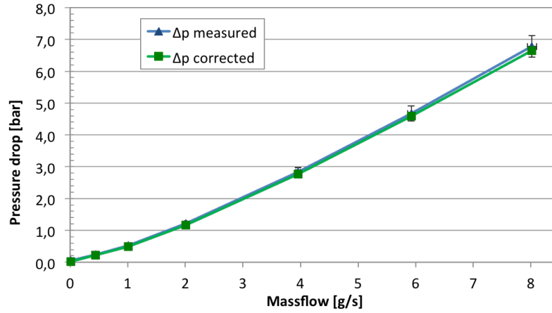
Figure 4.5: Measured and corrected pressure drop of the baseline cooling plate at -20\text{ }^{\circ}\text{C} set point temperature of the cooling plant. The error bars on the measured values are magnified 10 times to make them visible.
