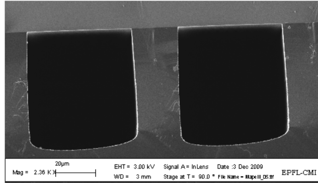
Figure 3.3: Magnification of a cross section cut through a cooling plate with 20 \mu\text{m} channel walls. The silicon wafer with channels is bonded to a Pyrex cover wafer. Courtesy of EPFL CMI
