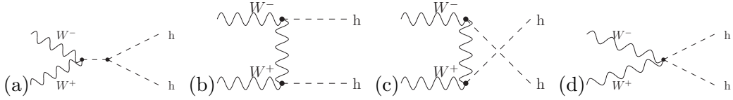
Figure 1. Four types of Feynman diagrams which contribute to the processes W^+W^- \rightarrow hh .
