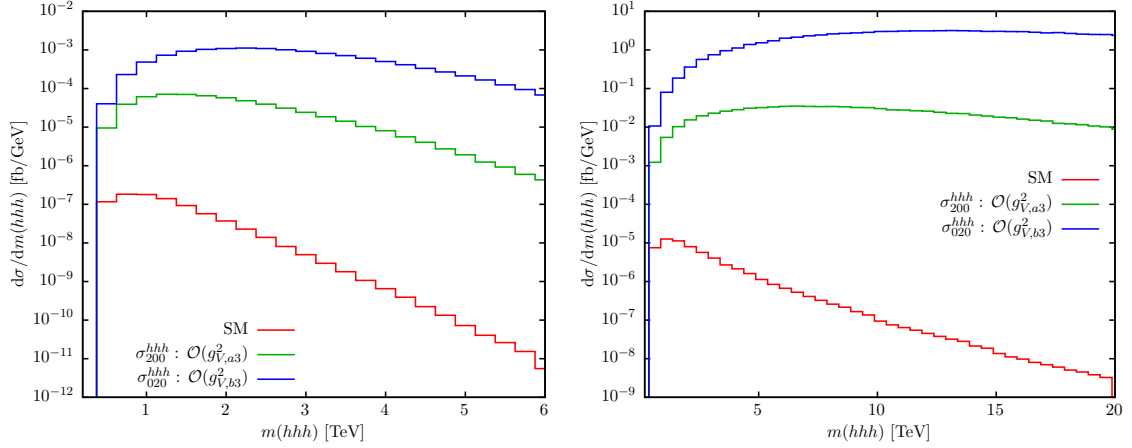
Figure 9. Triple-Higgs invariant mass distribution for the coefficients of the leading power corrections to VBF hhh production in pp collisions. We display results for 14 TeV (left) and for 100 TeV (right).
