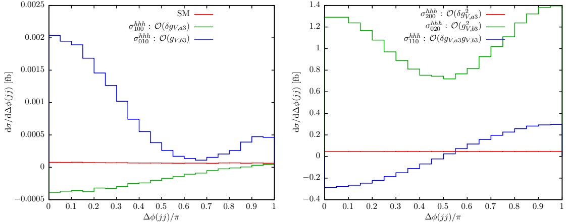
Figure 8. Distribution of \Delta\phi_{jj} for various modifications of VBF hhh production, at the 14 TeV LHC.
