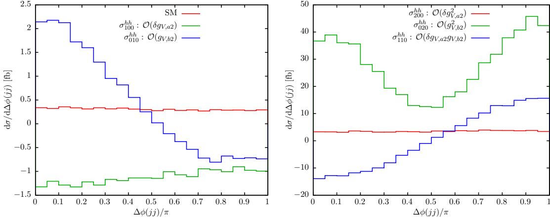
Figure 5. Distribution of \Delta\phi(jj) for various modifications of VBF hh production in the EFT, at the 14 TeV LHC.
