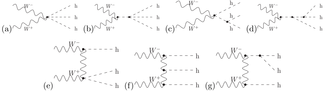
Figure 2. Seven types of Feynman diagrams which contribute to the processes W^+W^- \rightarrow hhh .
