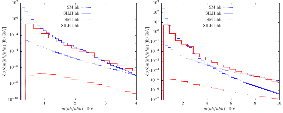
Figure 11. Maximally allowed enhancement of the differential cross section of VBF hhh production in pp collisions in the SILH model, as a function of the triple-Higgs invariant mass. We display results for 14 TeV (left) and for 100 TeV (right), identifying m(hhh) with the cutoff Q .
