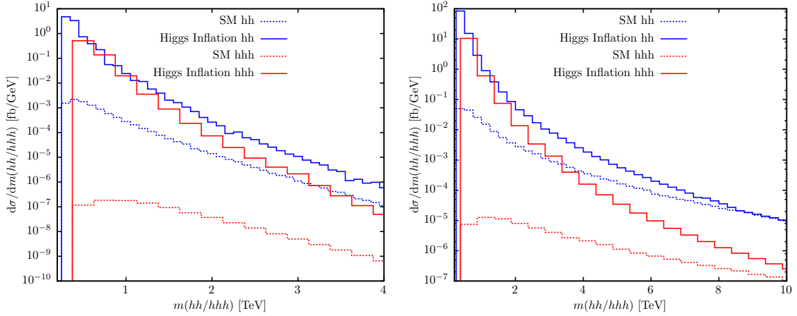
Figure 12. Maximally allowed enhancement of the differential cross section of VBF hhh production in pp collisions in the Higgs-inflation model, as a function of the triple-Higgs invariant mass. We display results for 14 TeV (left) and for 100 TeV (right), identifying m(hhh) with the cutoff Q .
