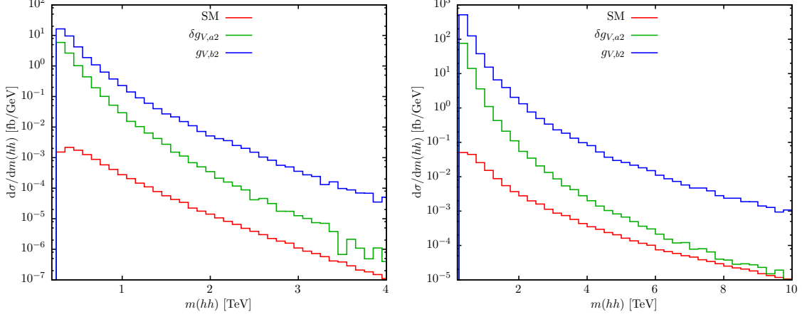
Figure 7. Maximally allowed enhancement of the differential cross section of VBF hh production in pp collisions, as a function of the Higgs-pair invariant mass. We display results for 14 TeV (left) and for 100 TeV (right), identifying m(hh) with the cutoff scale Q .
