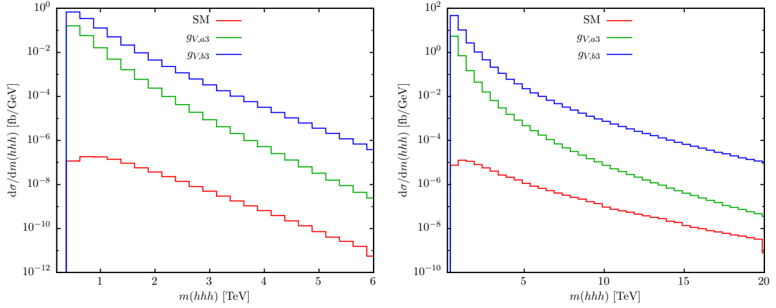
Figure 10. Maximally allowed enhancement of the differential cross section of VBF hhh production in pp collisions, as a function of the triple-Higgs invariant mass. We display results for 14 TeV (left) and for 100 TeV (right), identifying m(hhh) with the cutoff Q .
