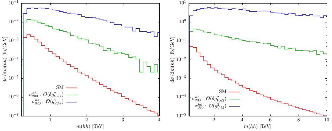
Figure 6. Higgs-pair invariant-mass distribution for the coefficients of the leading power corrections to VBF h h h production in pp collisions. The SM baseline is drawn in red. We display results for 14 TeV (left) and for 100 TeV (right).
