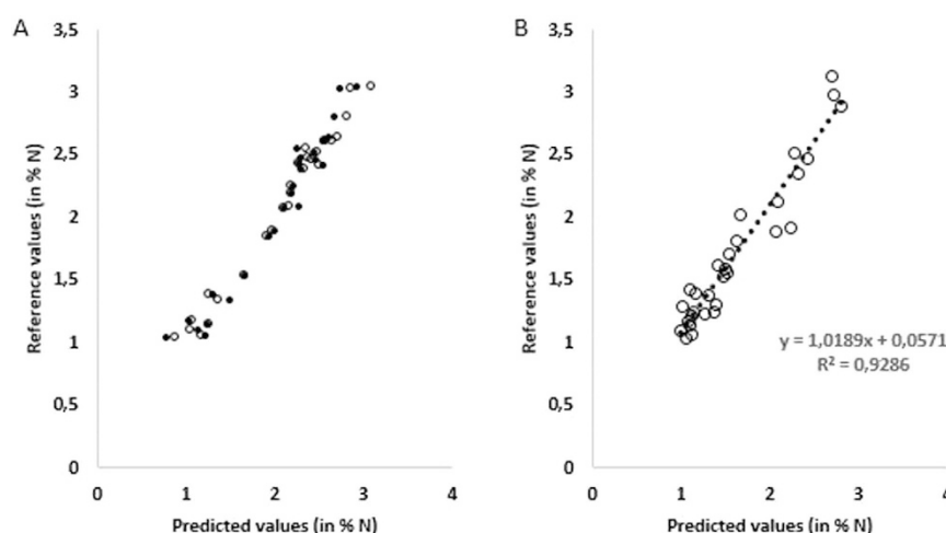
Figure 3. (A) Plot of % N in the Solanum lycopersicum L. samples analyzed in the calibration stage. Results of the reference values vs NIRM prediction (Model 3) are plotted. NIRM calibration (o) and cross-validation (·) results are displayed. (B) Plot of % N in the Solanum lycopersicum L. samples analyzed in the validation stage. Results of the reference values vs NIRM prediction (Model 3) are plotted.
