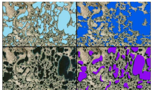
Figure 5. SAR-WBI (top left), MODIS Land/Water Mask (top right), Bing Maps (bottom left and background image in other panels) and the Global Lakes and Wetlands Database (bottom right) for Eskimo Lakes, Canada.
