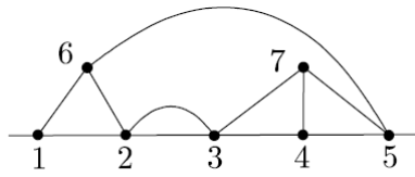
Figure 2.2: An admissible diagram
