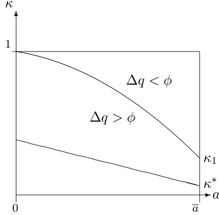
Figure 2: Price and quality differentiation
