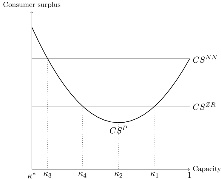
Figure 4: Consumer surplus under NN, ZR and P for \kappa_3 \geq \kappa^* .
