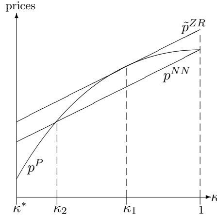
Figure 3: Prices under NN, ZR and P for \kappa_2 > \kappa^* .
