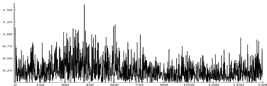
Figure 3: Absolute value of a series of returns produced by the microeconomic model.
