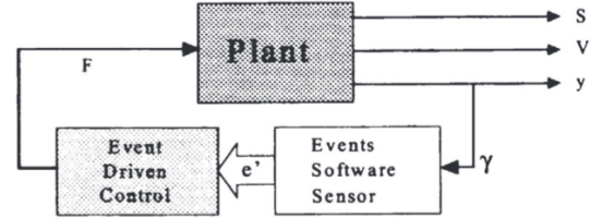
Figure 2. ED-TOC scheme
