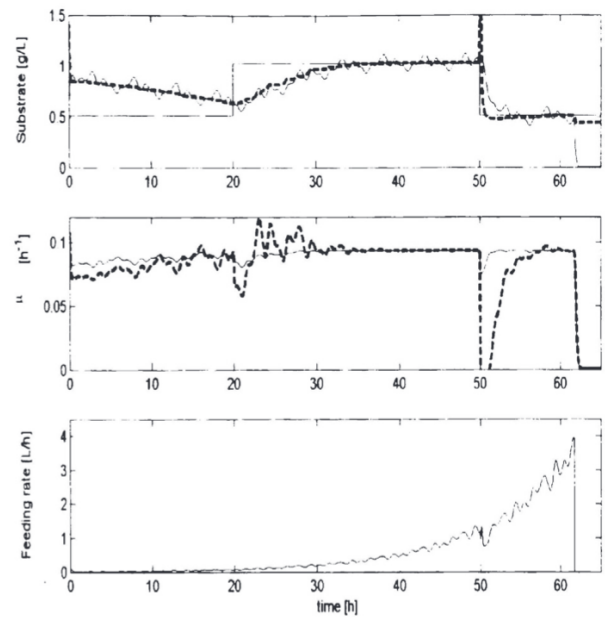
Figure 5: AES behavior for Scenario 6 in Table 2. In the substrate plot a step-like line shows S^* . Estimations are drawn with dashed lines.
