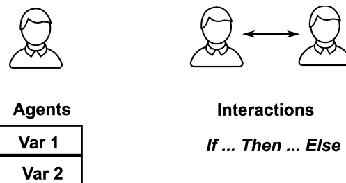
Figure 1 Agent-based methodology.
