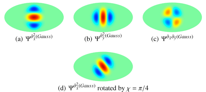
Figure 2. Mollweide projection of second Gaussian derivative wavelet on the sphere for wavelet half-width \theta_{hw} \simeq 0.4 rad. The rotated wavelet illustrated in panel (d) can be constructed from a sum of weighted versions of the basis wavelets illustrated in panels (a) through (c).
