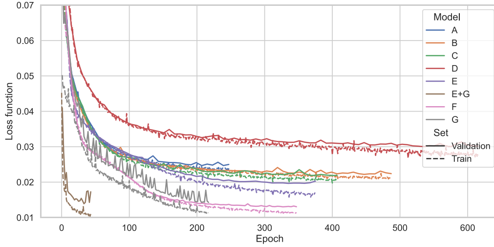
Fig. 4. Evolution of the loss function on the training and validation set for each model.
