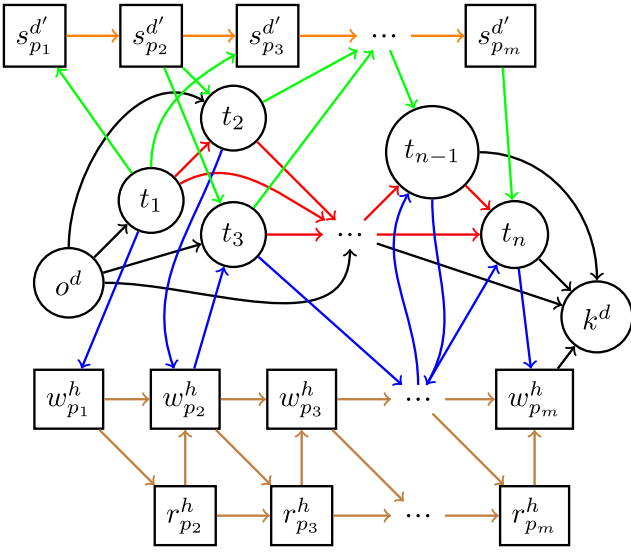
Fig. 2. Subproblem network G^d for depot d .
