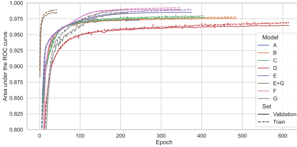
Fig. 5. Evolution of the ROC score on the training and validation set for each model.
