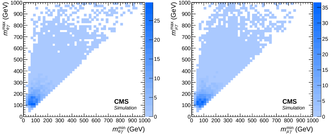
Figure 4: The two-dimensional distributions of m_{\ell\gamma}^{\max} versus m_{\ell\gamma}^{\min} of DY+ \gamma background events in the ee\gamma (left) and \mu\mu\gamma (right) channels, after the event selection, normalized to the cross section for DY+ \gamma production.
