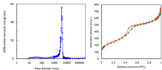
Figure 2. (Left) Size distribution of the macroscopic pore opening obtained by mercury intrusion porosimetry and (right) N_2 -sorption isotherms.
