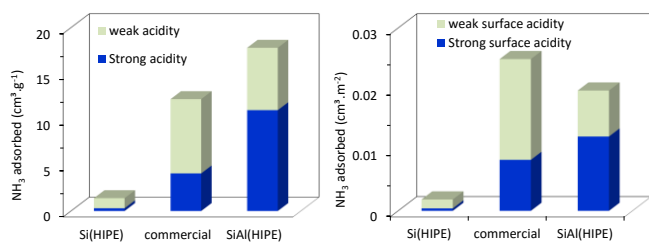
Figure 3. Acidity of SiAl(HIPE) measured by NH_3 -chemisorption 21 and compared to the commercial reference and to Si(HIPE). The acidity is expressed as the amount of NH_3 chemisorbed per gram of catalyst (left) or per m^2 of catalyst (right).
