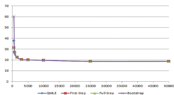
Figure 8: MSEs of all estimators under mixture of normals with \alpha = -0.1, \beta = 0.9, \gamma = 0.6, \theta = -0.2 .
