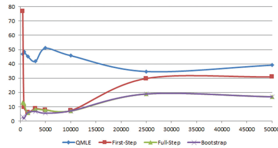
Figure 9: Bias of all estimators under t -distribution with 6 degrees of freedom, with \alpha = 0.1 , \beta = 0.9 , \gamma = 0.7 , \theta = -0.4 .
