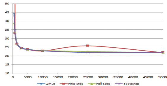
Figure 10: MSEs of all estimators under t -distribution with 6 degrees of freedom, with \alpha = 0.1 , \beta = 0.9 , \gamma = 0.7 , \theta = -0.4 .
