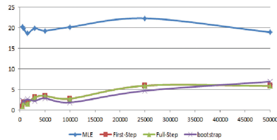
Figure 2: Bias of all estimators under normality with \alpha = -0.1, \beta = 0.9, \gamma = 0.6, \theta = -0.2 .
