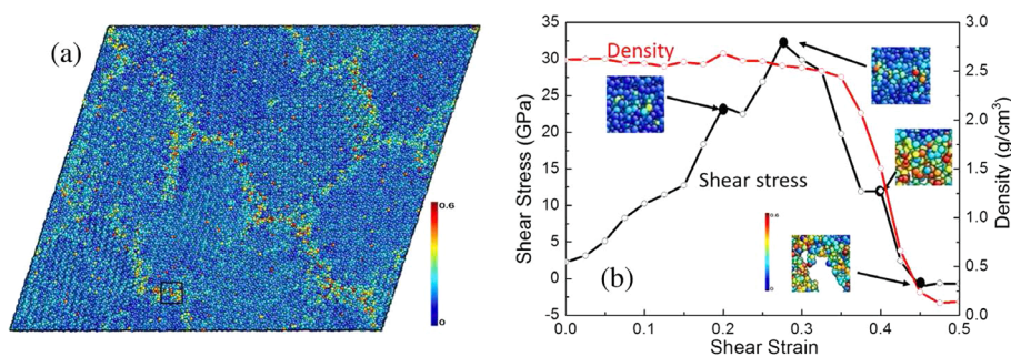
Fig. 14. Nanocrystalline Boron Carbide a) snapshot of a \text{B}_4\text{C} nano-aggregate at 0.325 shear strain. b) (b) Local shear-stress – shear-strain and density-shear-strain relations from a 1 \text{ nm} \times 1 \text{ nm} \times 1 \text{ nm} triple junction region (dark square in (a)). Some snapshots of critical states are extracted. Atoms are color coded based on the atomic shear strain. Guo et al. [52] with permission.
