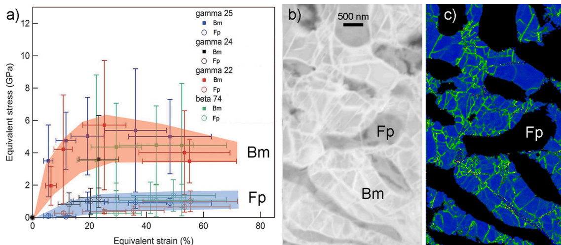
Fig. 12. Stress-induced amorphization in bridgmanite at high-pressure, high-temperature. a) Equivalent stress in bridgmanite (Bm) and ferropericlaase (Fp) as a function of strain. Deformation conditions are 2150 K, 27.5 GPa for gamma 25 and gamma 24; 2130 K, 27 GPa for gamma 22; 2000 K, 24.1 GPa for beta 74. Modified from Girard et al. [44] with permission. b) Sample gamma 21 (2130 K, 27 GPa) from Girard et al. [44]. Scanning precession electron diffraction virtual bright field where the amorphous lamellae in bridgmanite appear brighter than the crystalline parts (ferropericlaase appear even darker). c) Kernel Average Misorientation (KAM—third neighbor) from b) in bridgmanite (ferropericlaase not considered here appears in black). This representation highlights local gradients of orientation (in green). One can see that amorphous lamellae correlate with high KAM, demonstrating that they localize shear.
