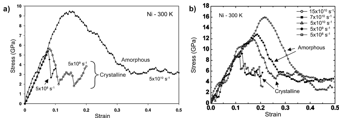
Fig. 20. Deformation of 2 nm × 2 nm Ni nanowires at 300 K – Strain rates are indicated in the figure. a) results from Ikeda et al. [65]. b) results from Branicio and Rino [16].
