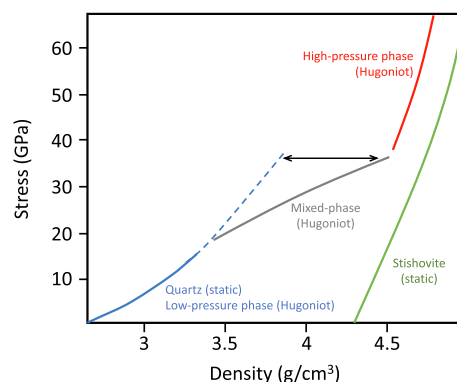
Fig. 1. Shock Hugoniot curve for quartz (adapted from [131]). Blue dashed line is an extrapolated equation of state fit to the 300 K quartz data. The 300 K static compression data for stishovite are represented by the green line.
