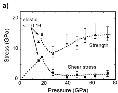
Fig. 10. Shock-induced amorphization of B_4C . a) Shear stress and strength of B_4C in the shocked state estimated from reshock and release experiments. After Vogler et al. [133] b) TEM observation of a fragment of B_4C produced by a ballistic test at a hypercritical impact velocity of 907 m/s (23.3 GPa). Misalignment of the lattice fringes on either side of the amorphous zone is highlighted by the lines and was measured to be 1^\circ , indicating shear. After [23] with permission.
