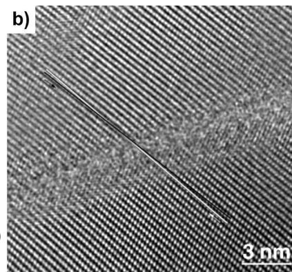
Fig. 10. Shock-induced amorphization of B_4C . a) Shear stress and strength of B_4C in the shocked state estimated from reshock and release experiments. After Vogler et al. [133] b) TEM observation of a fragment of B_4C produced by a ballistic test at a hypercritical impact velocity of 907 m/s (23.3 GPa). Misalignment of the lattice fringes on either side of the amorphous zone is highlighted by the lines and was measured to be 1^\circ , indicating shear. After [23] with permission.
