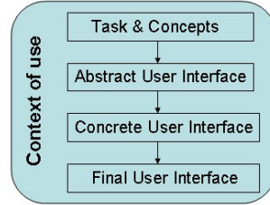
Fig. 1. The four levels of the Cameleon reference framework (source: [5]).
