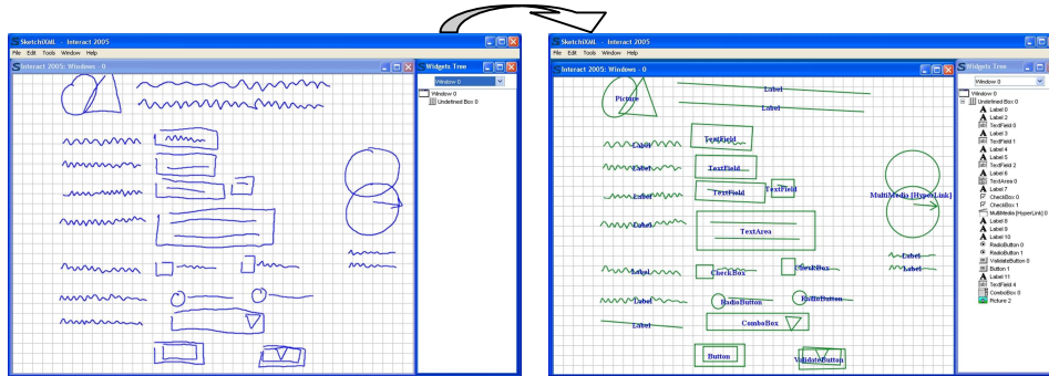
Fig. 6. SketchiXML workspace.
