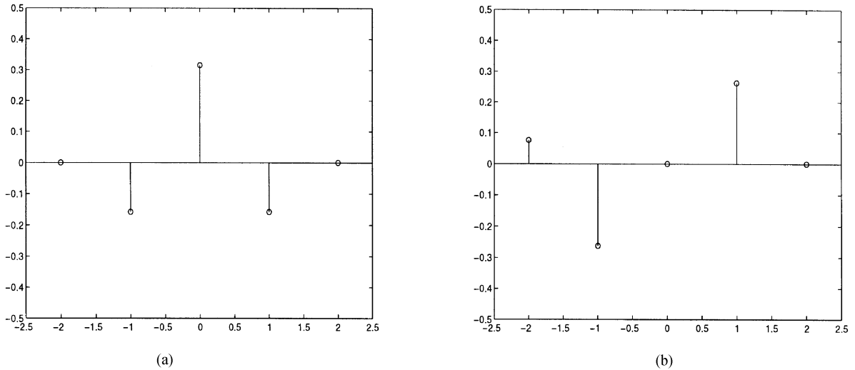
Fig. 6. (a) Real and (b) imaginary part of the samples of the edge detector filter.
