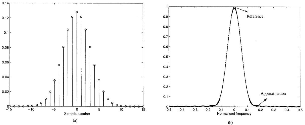
Fig. 3. Vertical factor ( g_2 ) of the perceptive analytic filter ( u_0 N = 0.15 \cdot N ): (a) filter actual samples in the spatial domain obtained as the inverse Fourier transform of the reference Gaussian function (see (b) and Eq. (8)); (b) 15 samples filter approximation.
