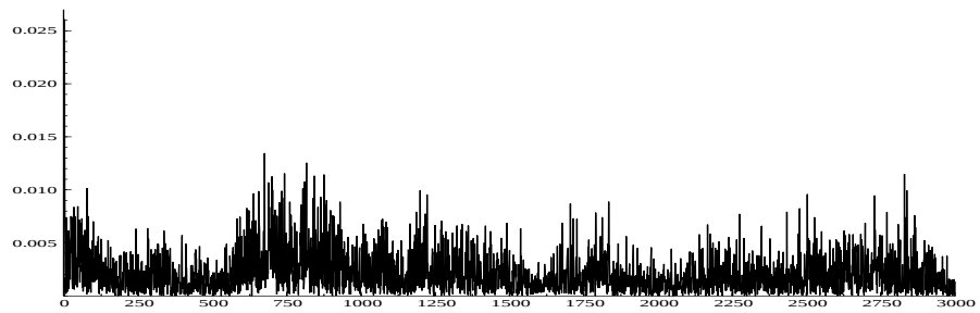
Figure 6: Series of simulated absolute returns |R_t|
