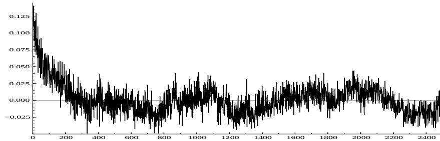
Figure 1: Autocorrelation function of the absolute returns |R_t| on Pound-Dollar
