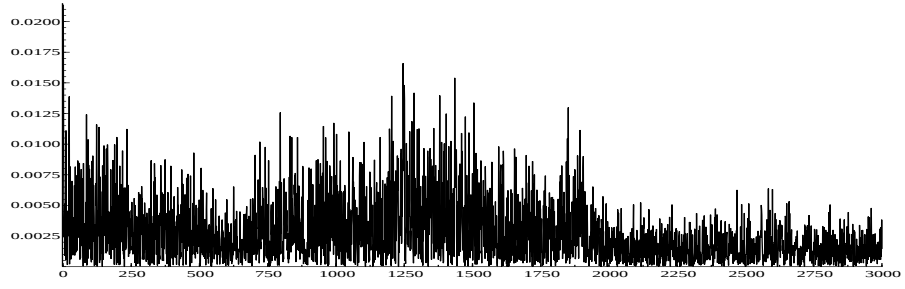
Figure 7: Series of simulated absolute returns |R_t|
