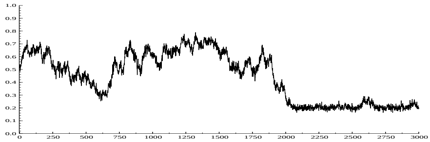
Figure 8: Evolution of the process k_t .
