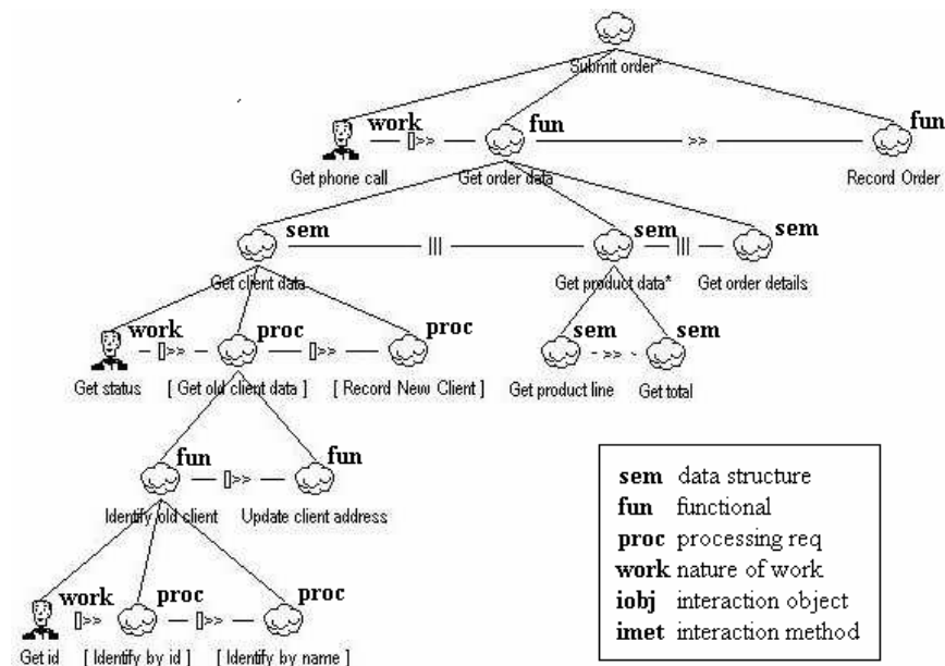
Figure 2 Goal hierarchy
