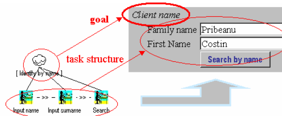
Figure 6 Interaction object group
