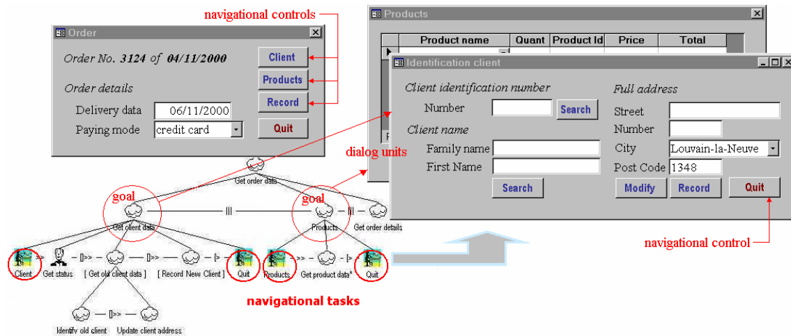
Figure 9 A task-based allocation
