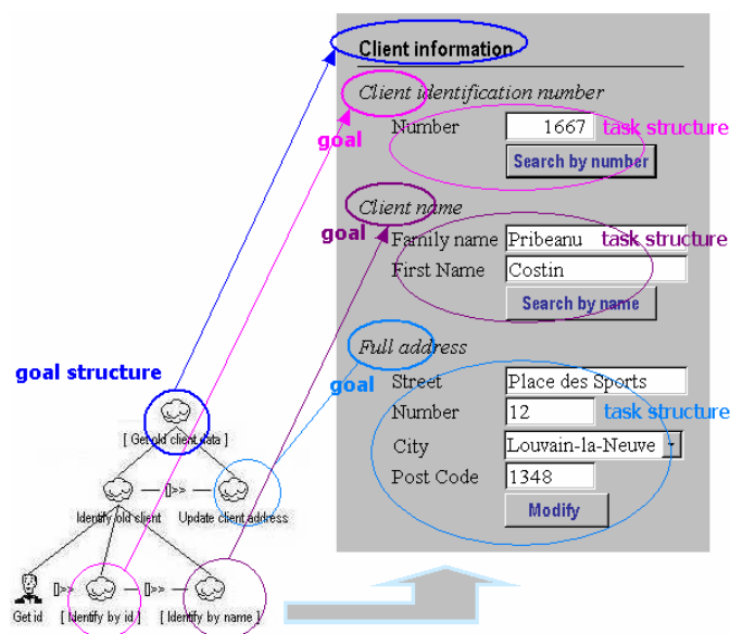
Figure 7 Higher level interaction object group
