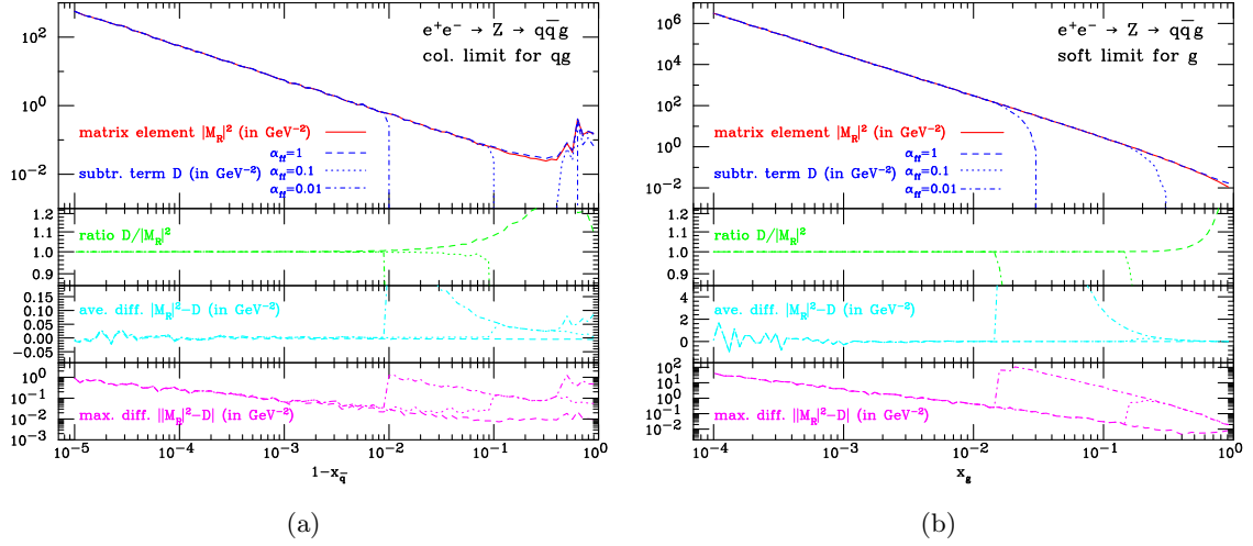
Figure 1: Matrix element squared |M_R|^2 (upper plots, solid line) and the subtraction terms D (upper plots, dashed/dotted/dot-dashed lines) for the process e^+(p_1)e^-(p_2) \rightarrow Z \rightarrow q(p_3)\bar{q}(p_4)g(p_5) as a function of 1 - x_{\bar{q}} = (p_3 \cdot p_5)/(p_1 \cdot p_2) and x_g = 1 - (p_3 \cdot p_4)/(p_1 \cdot p_2) in figures (a) and (b), respectively. Also plotted are the ratio D/|M_R|^2 , the difference |M_R|^2 - D (averaged over 100 random points per bin) and the maximal difference \max(|M_R|^2 - D) per bin. The dashed lines include the dipoles for each point in phase space, \alpha_{ff} = 1 , while for the dotted \alpha_{ff} = 0.1 and dot-dashed \alpha_{ff} = 0.01 the phase space for the dipoles has been restricted to the collinear/soft regions.
