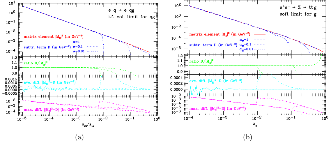
Figure 2: Matrix element squared |M_R|^2 (upper plots, solid line) and the subtraction term D (upper plots, dashed/dotted/dot-dashed lines) for (a) the process e^-(p_1)q(p_2) \rightarrow e^-(p_3)q(p_4)g(p_5) as a function of s_{25}/s_{12} = (p_2 \cdot p_5)/(p_1 \cdot p_2) and (b) the process e^+(p_1)e^-(p_2) \rightarrow Z \rightarrow t(p_3)\bar{t}(p_4)g(p_5) as a function of x_g = 1 - (p_3 \cdot p_4)/(p_1 \cdot p_2) . Also plotted are the ratio D/|M_R|^2 , the difference |M_R|^2 - D (averaged over 100 random points per bin) and the maximal difference \max(|M_R|^2 - D) per bin. The dashed lines include the dipoles for each point in phase space, \alpha = 1 , while for the dotted \alpha = 0.1 and dot-dashed \alpha = 0.01 the phase space for the dipoles has been restricted to the collinear/soft regions.
