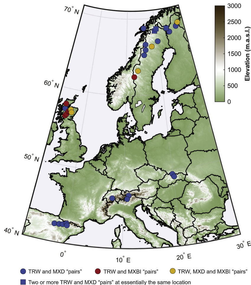
Fig. 1. Map showing the location of the temperature-sensitive tree-ring data. The colour-coded symbols indicate "pairs" of TRW, MXD, and MXBI data. Square symbols indicate two or more TRW and MXD "pairs" from essentially the same location.
