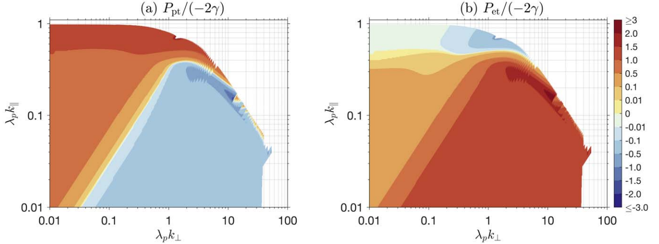
Figure 2. Total energy transfer rates in k_\perp - k_\parallel space: (a) the proton energy transfer rate P_{pt} normalized by (-2\gamma) , and (b) the electron energy transfer rate P_{et} normalized by (-2\gamma) .
