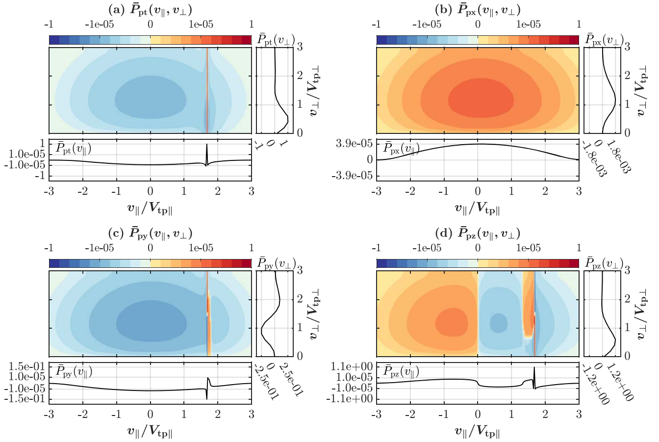
Figure 9. The 1D and 2D distributions of proton energy transfer rates in Case 3, where \lambda_{p\parallel} = 0.01 and \lambda_{p\perp} = 0.5 . The description of panels (a)–(d) is the same as that in Figure 4.
