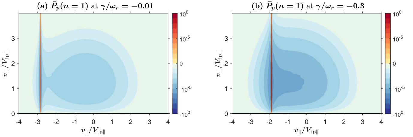
Figure 14. The v_{\parallel} – v_{\perp} distributions of proton energy transfer rates at n = 1 for parallel-propagating Alfvén-mode waves in a \beta_p = 30 plasma: (a) the wave having \lambda_p k = 0.06 , \omega_r/\Omega_{cp} \simeq 0.03 , and \gamma/\omega_r = -0.01 ; and (b) the wave having \lambda_p k = 0.09 , \omega_r/\Omega_{cp} \simeq 0.03 , and \gamma/\omega_r = -0.3 . The data are normalized by the maximum in each distribution.
