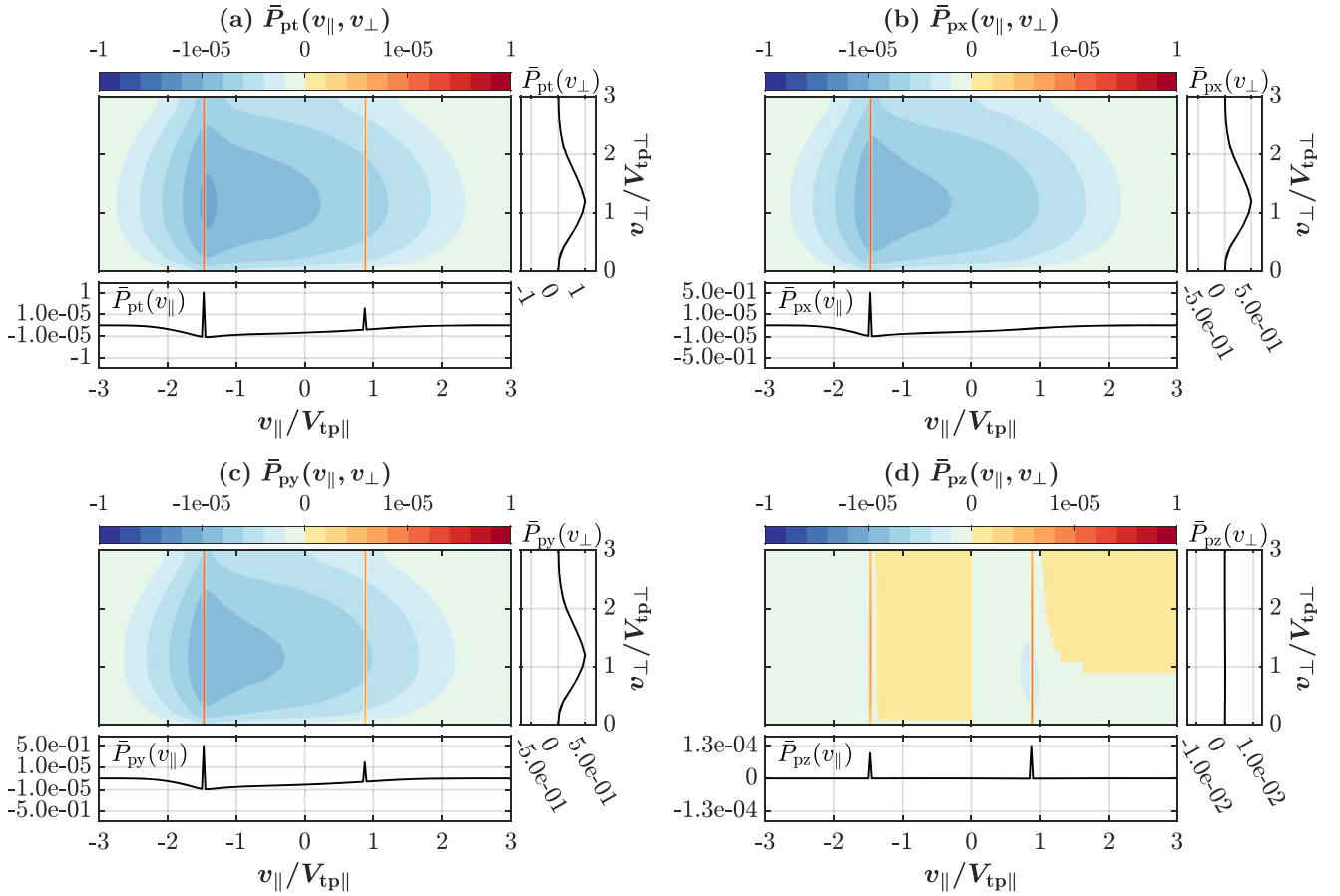
Figure 7. The 1D and 2D distributions of proton energy transfer rates in Case 2 where \lambda_{p\perp} = 0.01 and \lambda_{p\parallel} = 0.7 . The description of panels (a)–(d) is the same as that in Figure 4.
