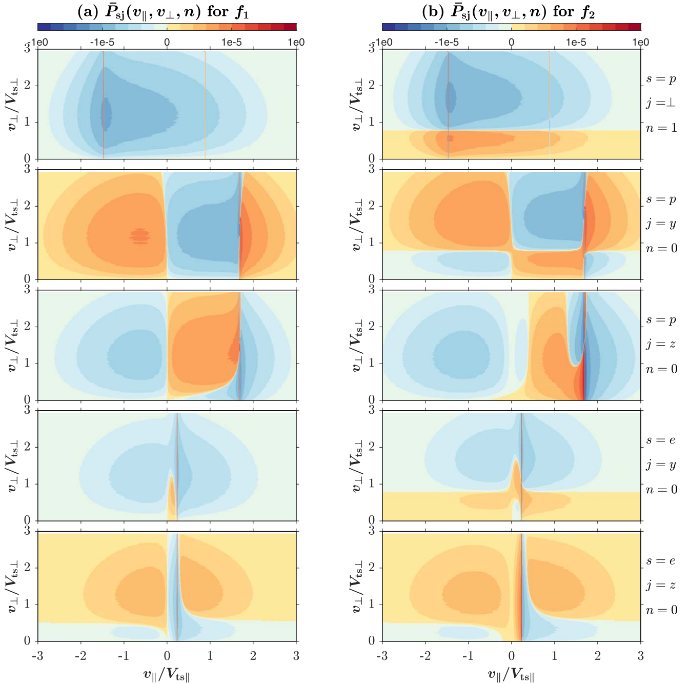
Figure 13. A comparison between two different wave-particle correlation functions: (a) f_1 = q_s \mathbf{E}_1 \cdot \mathbf{v} f_{s1} and (b) f_2 = -q_s v^2 \mathbf{E}_1 \cdot \partial_{\mathbf{v}} f_{s1} / 2 . (Upper panels) \bar{P}_{p\perp}(v_{\parallel}, v_{\perp}, n = 1) in Case 2; (second panels) \bar{P}_{py}(v_{\parallel}, v_{\perp}, n = 0) in Case 3; (third panels) \bar{P}_{pz}(v_{\parallel}, v_{\perp}, n = 0) in Case 3; (fourth panels) \bar{P}_{ey}(v_{\parallel}, v_{\perp}, n = 0) in Case 4; and (bottom panels) \bar{P}_{ez}(v_{\parallel}, v_{\perp}, n = 0) in Case 4.
