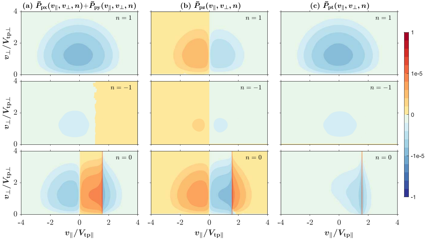
Figure 5. The v_{||}-v_{\perp} distributions of proton energy transfer rates at n = \pm 1 and n = 0 in Case 1: (a) the perpendicular energy transfer rate, P_{px} + P_{py} ; (b) the parallel energy transfer rate, P_{pz} ; and (c) the total energy transfer rate, P_{pt} . The data are normalized by the maximum P_{pt} in the v_{||}-v_{\perp} plane.
